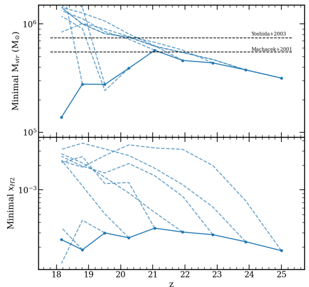
Fig. 9. Minimum mass (top) and minimum x_{\text{H}_2} fraction (bottom) of halos hosting clumps in our simulation as a function of redshift. The blue solid lines show the evolution of these minimums and the dashed lines show the subsequent mass or x_{\text{H}_2} evolution of the relevant 'minimal' halo, usually increasing in both mass and \text{H}_2 fraction. In the top panel, the horizontal lines show the critical mass found by Yoshida et al. (2003) and Machacek et al. (2003) .
