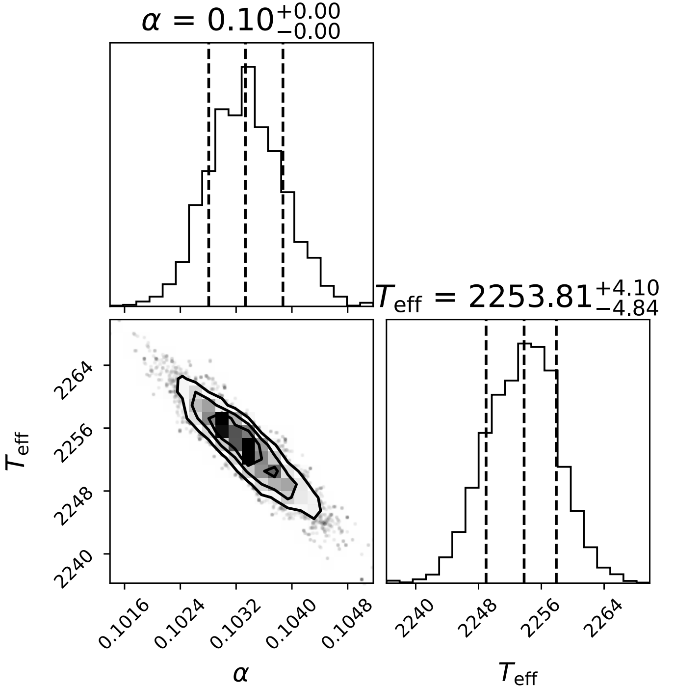
Fig. C.1. Corner plot from the fitting process of T_{\text{eff}} and the scale parameter \alpha (Section 3.3), for J0304-2435.
