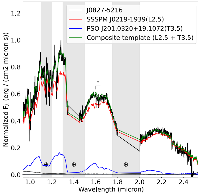
Fig. 7. Spectrum of J0827-5216 and template spectra of its component, a L2.5 (red) and a T3.5 (blue), as well as their composite template (green). The H-dip caused by methane absorption of the T dwarf atmosphere is indicated by the star symbol.
