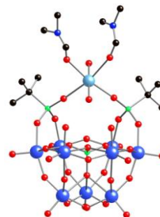
Figure 4. Structure of the anion [\text{PW}_9\text{O}_{34}\{\text{P}(\text{O})t\text{Bu}\}_2\{\text{Ca}(\text{H}_2\text{O})_2(\text{dmf})_2\}]^{3-} (5)
