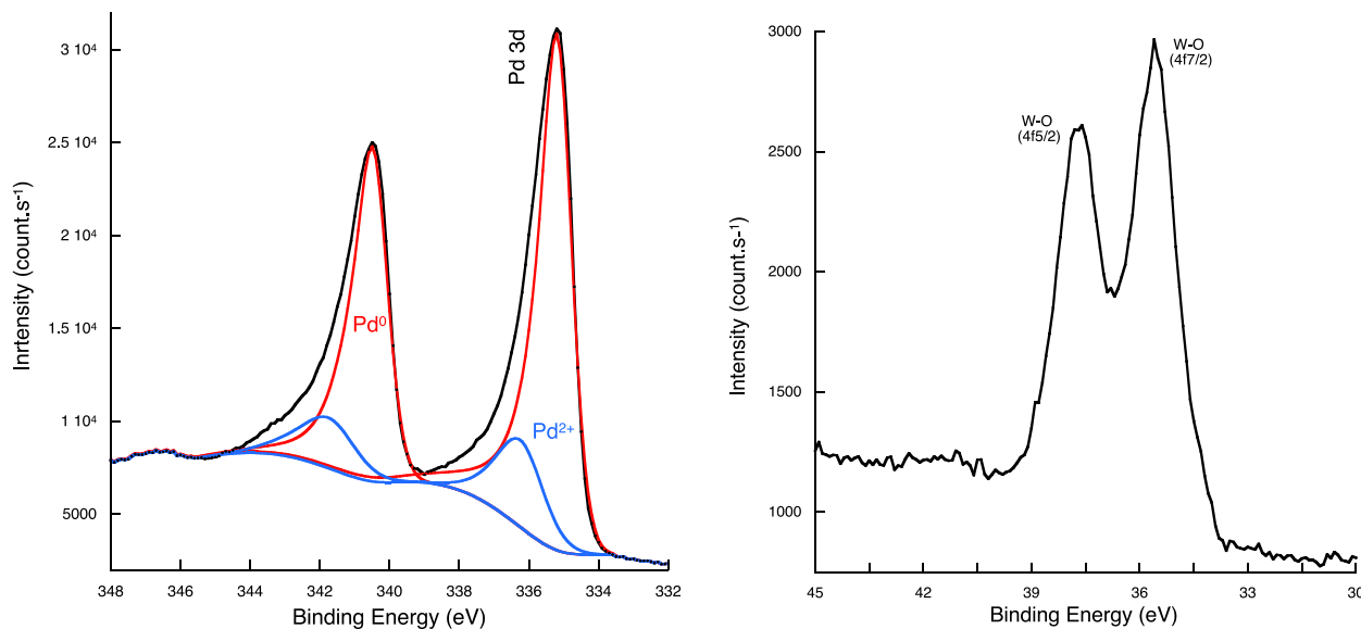
Fig. 8: High resolution Pd3d (left) and W4f (right) spectra of a solid sample of Pd 0 NPs stabilized by [PW 11 O 39 ] 7- anions prepared by precipitation and filtration of NPs obtained by reduction of a highly concentrated solution of compound 3 (initial concentration of 3 = 5.10 -3 mol L -1 ).
