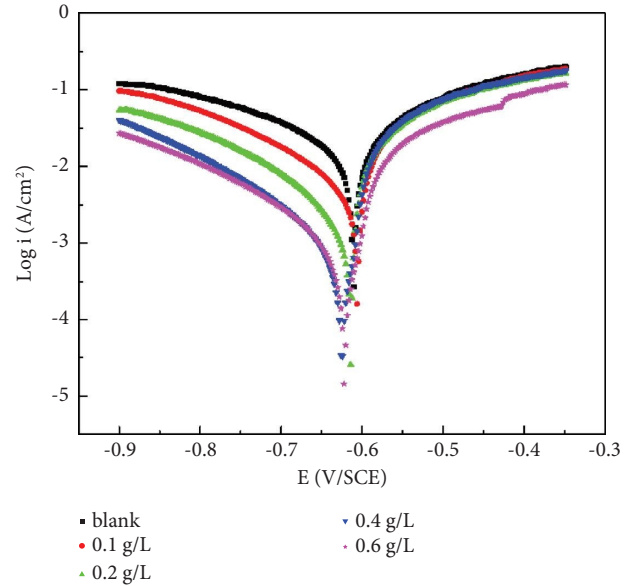
FIGURE 3: Polarization curves of Al 2024 alloy electrode in 1.0 M HCl in the presence and absence of different concentration of AHA extract at 298 K.
