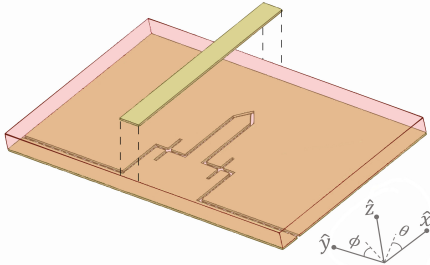
Fig. 4. DC Block placed on the ground plane to separate the signal from the CPW feeding the PDs.
