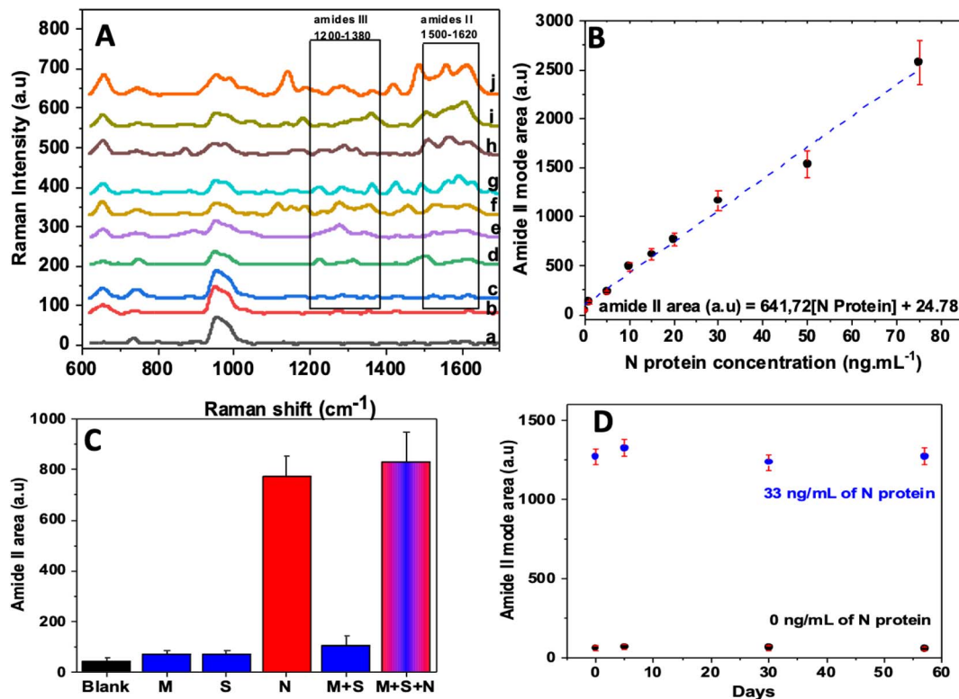
Fig. 4 (A) SERS spectra of bioSERS chip aptamer/cysteamine/AgNPs/SiNWs in the presence of different protein concentrations 1 \text{ ng mL}^{-1} (c), 5 \text{ ng mL}^{-1} (d), 10 \text{ ng mL}^{-1} (e), 15 \text{ ng mL}^{-1} (f), 20 \text{ ng mL}^{-1} (j), 30 \text{ ng mL}^{-1} (h), 50 \text{ ng mL}^{-1} (i) and 75 \text{ ng mL}^{-1} (j). (B) calibration plot displaying the amide II mode ( 1500 to 1630 \text{ cm}^{-1} ) area versus the concentration of the target protein. (C) Analytical response of the aptasensor toward different proteins: N ( 33 \text{ ng mL}^{-1} ), S ( 33 \text{ ng mL}^{-1} ) and M ( 33 \text{ ng mL}^{-1} ); amide II mode area for each type of analyte. (D) Storage stability of the aptasensor stored for 57 days at 4 \text{ }^\circ\text{C} and its response in presence of 33 \text{ ng mL}^{-1} of N protein recorded periodically.
