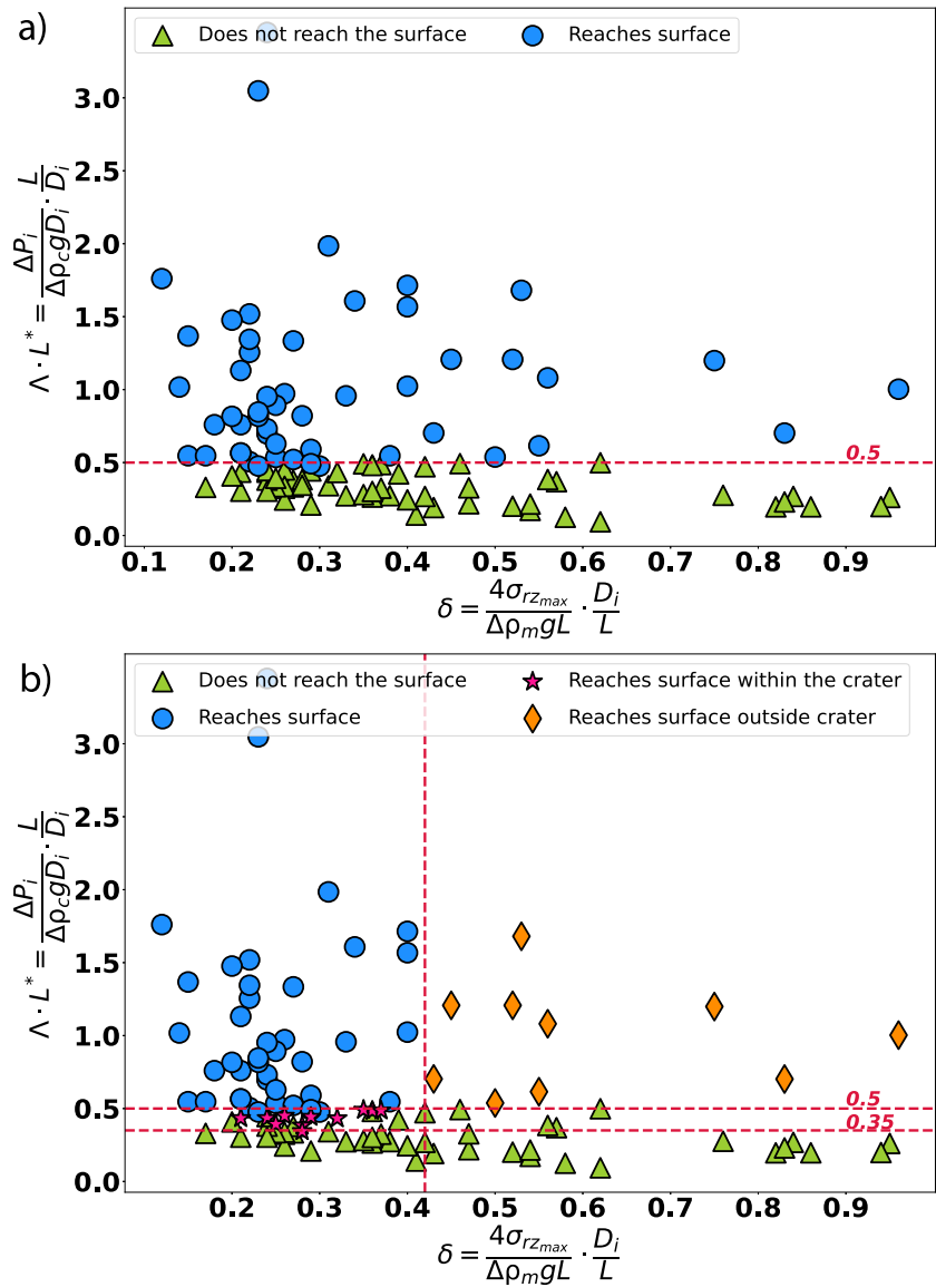
Figure 10. Regime diagram for the 2D propagation of magma dykes in an unloading stress field caused by a crater topography in the parameter space \Delta L^* as a function of \delta . (a) Behavior for control dykes. Blue dots: control dykes reach the surface, green triangles: control dykes do not reach the surface. (b) Behavior for all dykes. Blue dots: dykes reach the surface everywhere; pink stars: dykes reach the surface only within the crater; orange diamonds: dykes reach the surface only outside the crater; green triangles: dykes remain stored at depth everywhere. Reaching or not the surface for a dyke is controlled by the parameter \Delta L^* , while the deviation of the dyke is controlled by the parameter \delta . As a consequence, the region of this parameter space for which dykes reach the surface only within the crater is quite narrow ( 0.35 < \Delta L^* < 0.5 and \delta < 0.42 ).
