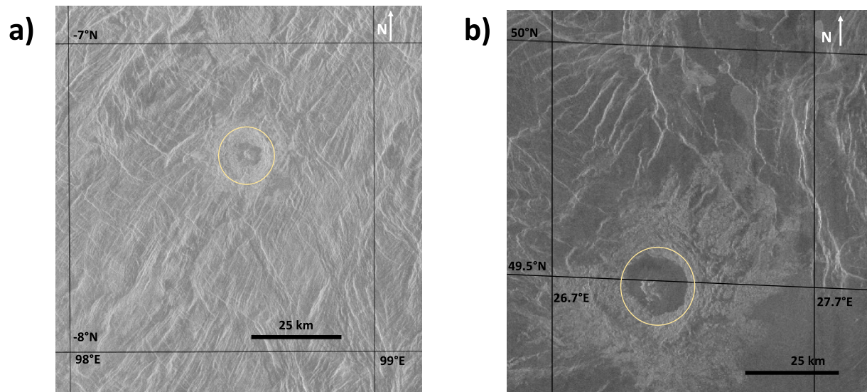
Figure 1. Examples of dark-floored craters and their highly deformed surroundings: (a) Chloe and (b) Kauffman (see topographic profiles in Figure 2).
