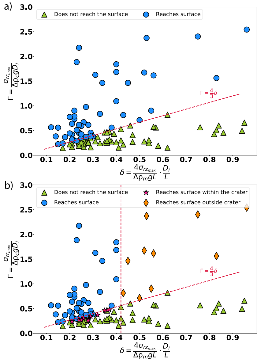
Figure 9. Regime diagram for the 2D propagation of magma dykes in an unloading stress field caused by a crater topography in the parameter space \Gamma as a function of \delta . (a) Behavior for control dykes. Blue dots: control dykes reach the surface, green triangles: control dykes do not reach the surface. (b) Behavior for all dykes. Blue dots: dykes reach the surface everywhere; pink stars: dykes reach the surface only within the crater; orange diamonds: dykes reach the surface only outside the crater; green triangles: dykes remain stored at depth everywhere.
