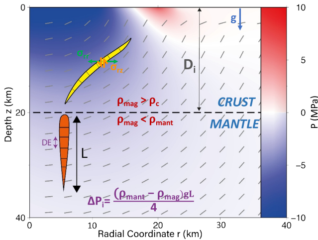
Figure 7. Schematic for the dyke propagation model in an external stress field adapted from Maccaferri et al. (2011). The dyke of length L is composed of a succession of n dislocation elements of length l . This model considers the stress balance at the center of each of these elements to test for dyke propagation. The different stress components \sigma_{rr} and \sigma_{zz} acting on the opening/closing and deviation of the dyke are represented. The color scale represents the pressure perturbation caused by the unloading (a crater topography of radius R = 20 km in that case) and the dashes exterior to the cracks, the direction of the maximum compressive stress \sigma_1 . The dyke initially starts in the mantle with an overpressure \Delta P_i (orange dyke) and propagates until it reaches its final state (yellow dyke). The case of a crack starting at the lateral position R/4 is represented.
