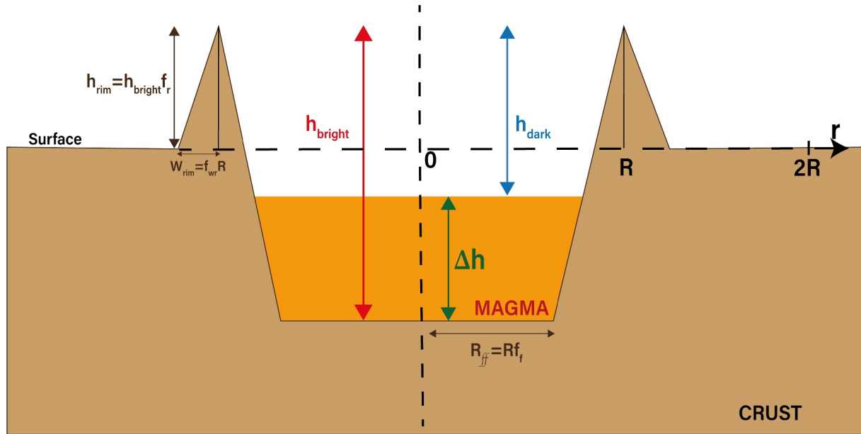
Figure 5. Schematic of a truncated cone-shaped crater with a rim. The thickness of the partial infilling of a crater by lavas \Delta h , corresponding to the difference in depth between bright-floored and dark-floored craters h_{\text{bright}} - h_{\text{dark}} , is represented. Quantities h_{\text{rim}} , R_{\text{ff}} and W_{\text{rim}} are also represented.
