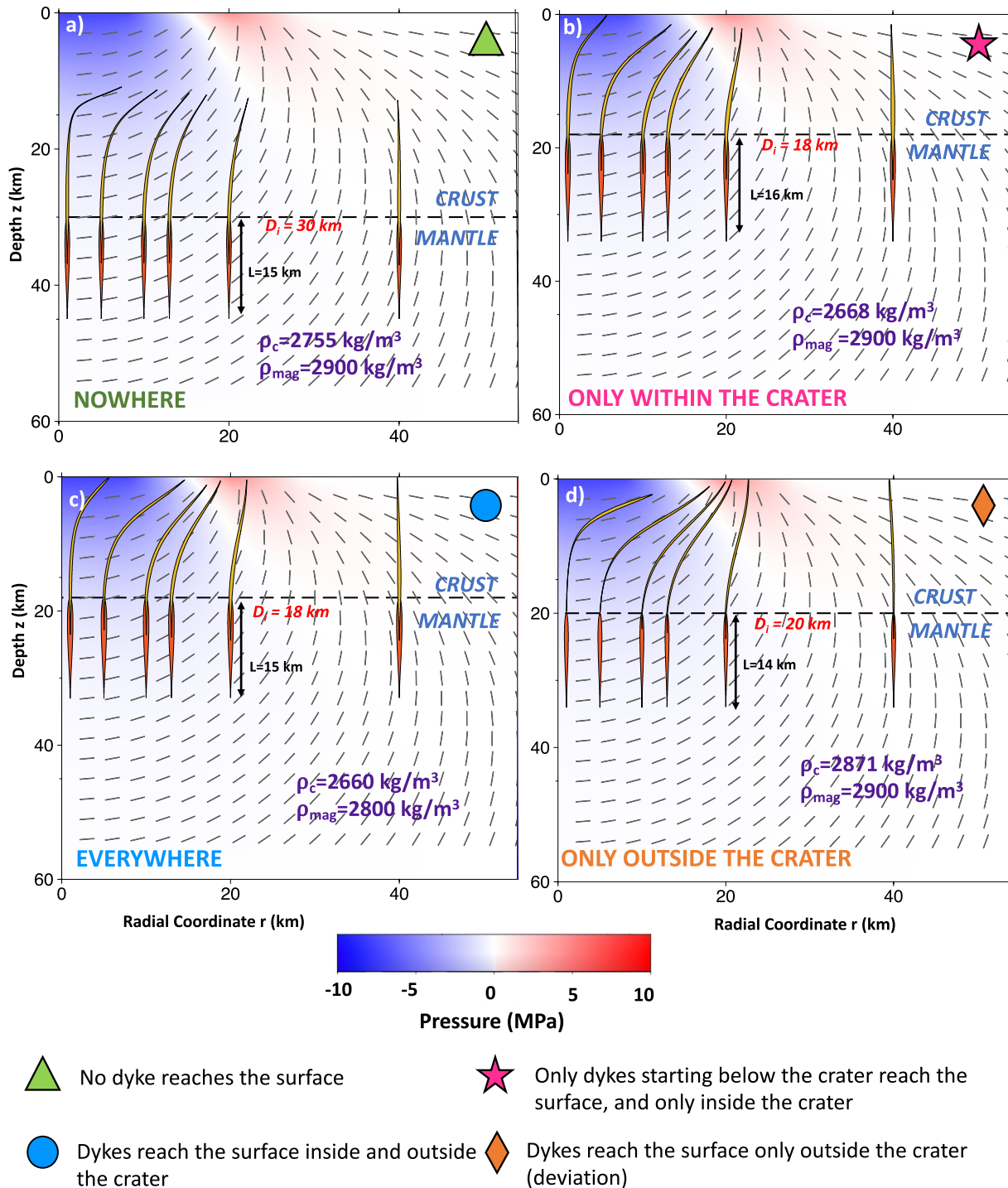
Figure 8. Four typical propagation behaviors for magma-filled cracks below a crater of radius R = 20 \text{ km} . For each example, two dykes are represented: the initial state with the upper tip at the crust/mantle transition (orange dyke), and the final stage of the dyke when its propagation is complete (yellow dyke). The dykes can either remain stored at depth (green triangles), reach the surface only within the crater (pink stars), reach the surface both inside and outside the crater (blue dots) or reach the surface only outside the crater (orange diamonds). Several parameters vary: initial depth D_i , crust density \rho_c , magma density \rho_{\text{mag}} and the initial length of the dyke L . Gray dashed lines indicate the direction of maximum compressive stress \sigma_1 and background color-scale is the pressure perturbation caused by the unloading P (MPa). Values of E , \mu , \lambda , and g used for these simulations are given in Table 2.
