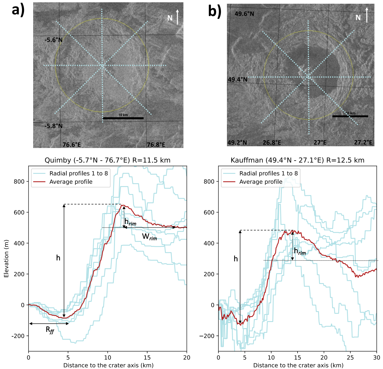
Figure 2. Two examples of craters: (a) Quimby a bright-floored crater and (b) Kauffman a dark-floored. Top: Magellan Synthetic Aperture Radar images and profiles drawn from JMars. Bottom: topographic profiles obtained from the stereo map of Venus (in blue) (Herrick et al., 2012) with the average profile derived from these data (in red) and the measured depth of crater h , the rim height h_{rim} , the rim width W_{rim} and the flat floor radius R_{ff} for Quimby crater. Rim height corresponds to the difference between the highest point of the rim (dashed line) and the level of the surrounding terrain (dotted line) at 3 radii of the crater center as in Herrick et al. (1997).
