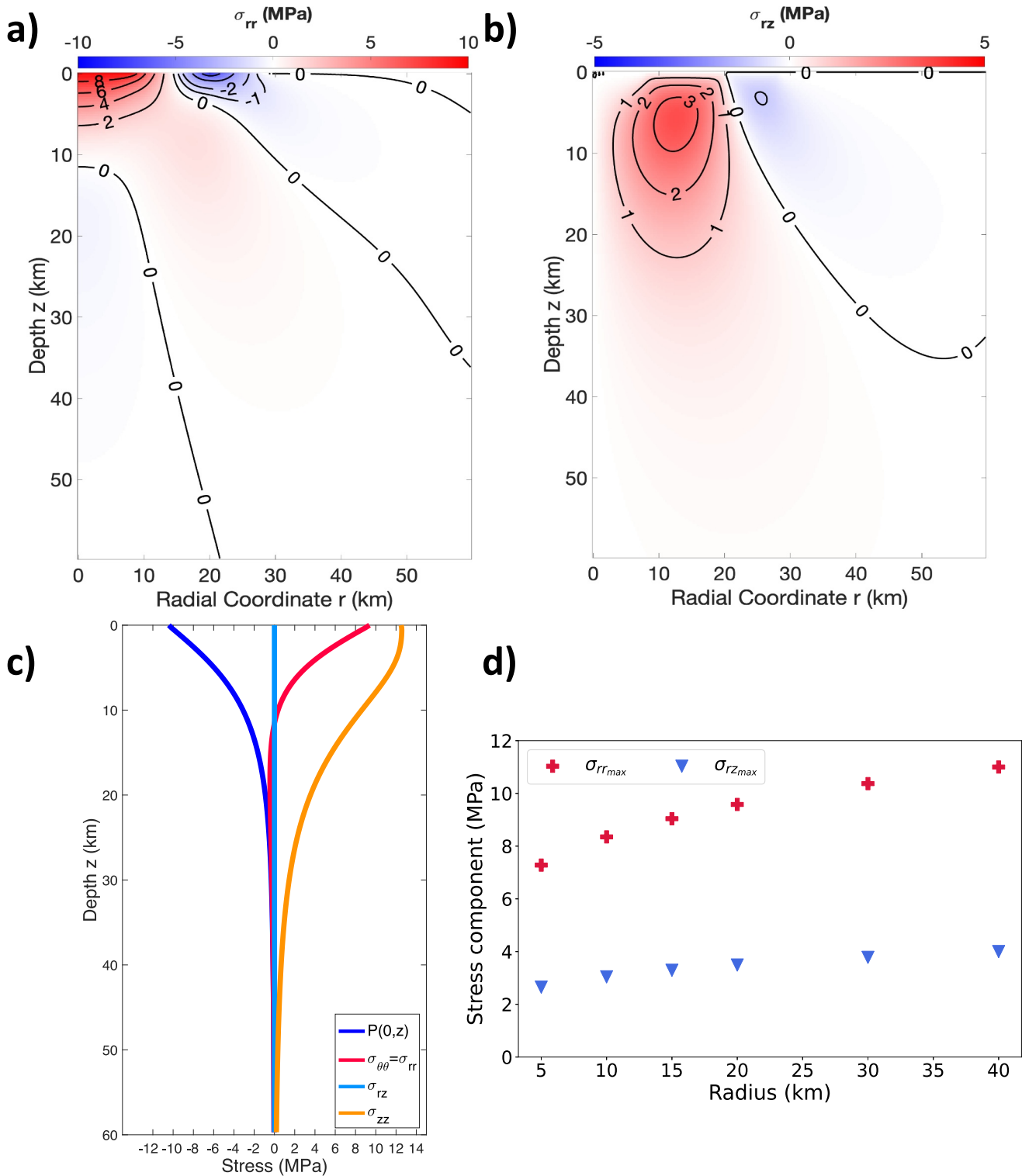
Figure 6. Radial and non-diagonal stress perturbations \sigma_{rr} and \sigma_{rz} caused by a crater unloading of topography h(r) (Equation 6) at the surface of a semi-infinite medium, with R = 20 km and h_{\text{bright}} = 780 m. Tension is positive. (a) Radial stress \sigma_{rr} , varying between -2 and 9 MPa. (b) Shear stress on the coordinate planes \sigma_{rz} , varying between -1 and 4 MPa. (c) Stress components \sigma_{rr}(0, z) , \sigma_{rz}(0, z) , \sigma_{\theta\theta}(0, z) , \sigma_{zz}(0, z) , and pressure perturbation P(0, z) at the axis of the unloading. (d) Maximum values of \sigma_{rr} (red crosses) and \sigma_{rz} (blue triangles) for crater radii ranging from 5 to 40 km. The ratio \sigma_{rz_{max}}/\sigma_{rr_{max}} remains approximately constant and equal to 0.36 while varying the crater radius. The parameters used to calculate this stress field are given in Table 2.
