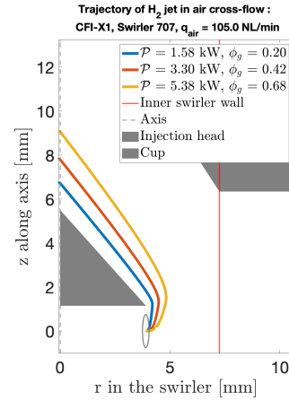
Figure 2: Simulation of the hydrogen jet trajectory for three different equivalence ratios: 0.20 ( J = 0.03 ), 0.42 ( J = 0.13 ) and 0.68 ( J = 0.35 ).
