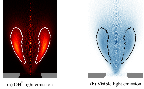
Figure 7: Abel-inverted images of the light radiated in a lifted thin flame ( \mathcal{P}_{th} = 4.6 kW and \phi_g = 0.42 ) (a) by \text{OH}^* radicals and (b) in the visible range. The contour of the Abel transformed \text{OH}^* image obtained with Otsu method is superimposed on both images.
