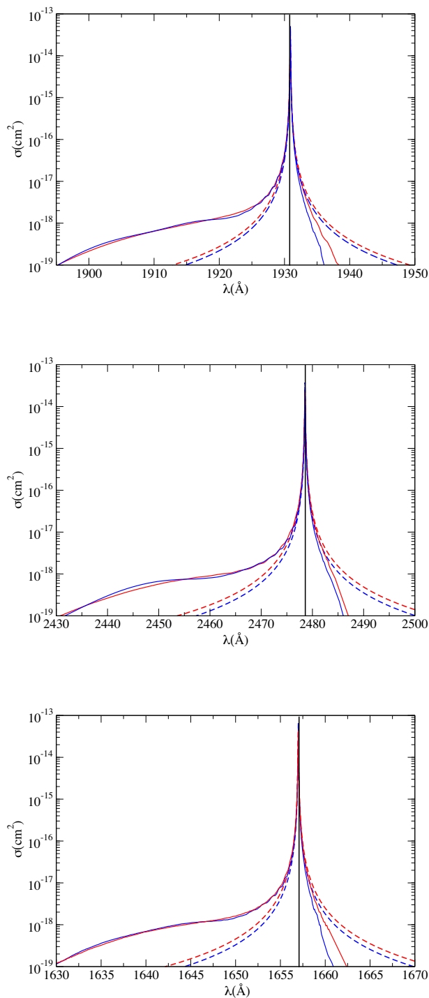
Figure 9. Temperature dependence of C 1930 (top), C 2478 (middle), and C 1657 (bottom) lines perturbed by He collisions. T = 10000 K (red lines) and T = 5000 K (blue lines). n_{\text{He}} = 2 \times 10^{19} \text{ cm}^{-3} . Lorentzian lines are reported in dashed lines. A vertical dark line shows the position of the unperturbed lines.
