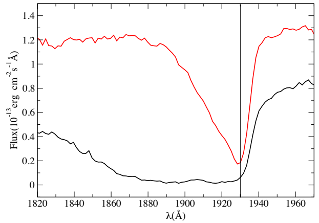
Figure 11. Top: density dependence of the 1930 line profile for He density varying from 2 to 5 \times 10^{21} \text{ cm}^{-3} . Bottom: IUE spectrum of L145-141 (Weidemann et al. 1980, black curve) and LDS687A (Oswalt et al. 1991, red curve).
