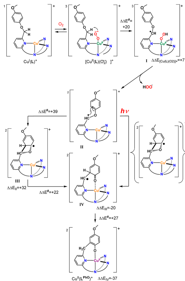
Scheme 1. Mechanistic Proposal. \Delta\Delta E (kcal/mol, PBE0-D3/def2-ZTVP) are Electronic Energy Differences Relative to the Previous Minimum, Indicated as a Subscript. \Delta\Delta E^\ddagger (kcal/mol) are Energy Barriers
