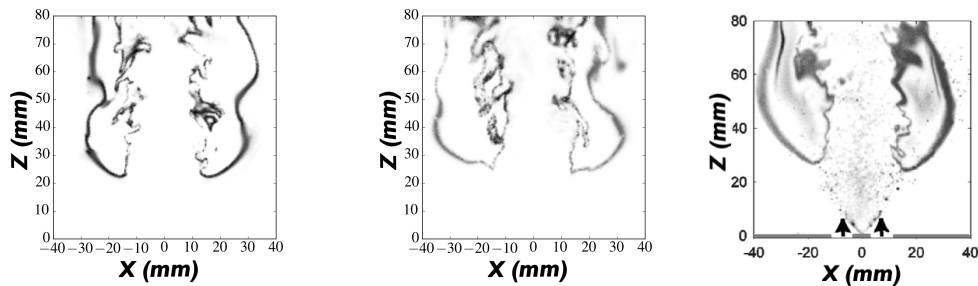
Fig. 7 Instantaneous normalized OH mass fraction (Case A: left, case B: middle). Experiments (right): instantaneous OH-PLIF shot, from [14].
