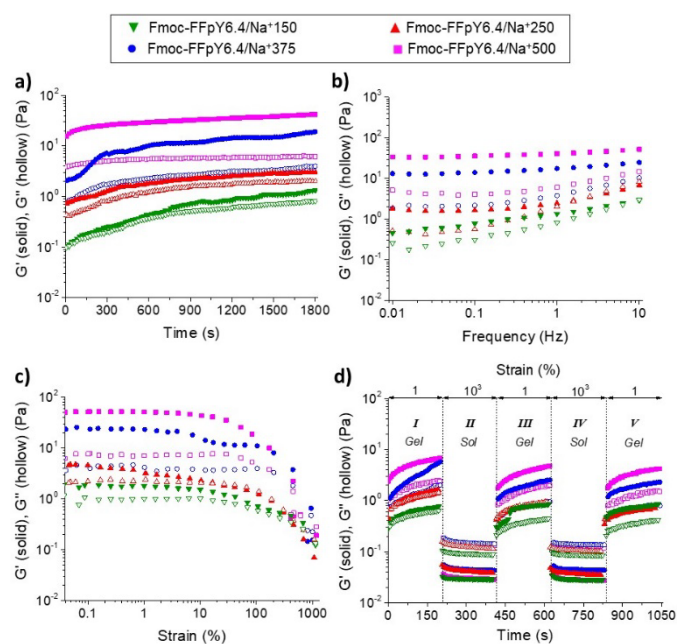
Fig. 5 Rheological properties of Fmoc-FFpY6.4/Na + hydrogels prepared in 150 ( \nabla ), 250 ( \blacktriangle ), 375 ( \bullet ), and 500 mM ( \blacksquare ) NaCl. Storage modulus ( G' - solid symbols) and loss modulus ( G'' - hollow symbols) as a function of the (a) time (1 Hz, 1% strain), (b) frequency (0.01–10 Hz, 1% strain), (c) strain (0.01–1000%, 1 Hz), and (d) dynamic step strain amplitude tests (1% or 1000% strain) at 20 °C.
