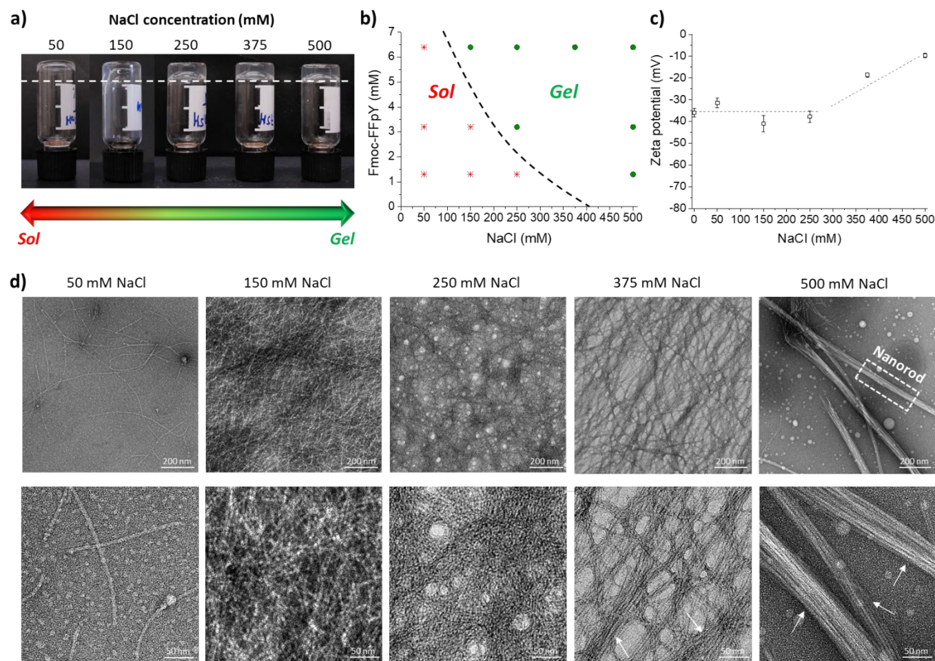
Fig. 1 (a) Inverted tube tests of supramolecular Fmoc-FFpY6.4/Na + hydrogels formed after 24 h, at a fixed Fmoc-FFpY concentration of 6.4 mM. (b) Phase diagram of Fmoc-FFpY/Na + mixtures in molar concentration. (c) Zeta potential of Fmoc-FFpY6.4 hydrogels as a function of NaCl concentration. Dashed lines are a guide to the eye. (d) TEM micrographs of negatively stained Fmoc-FFpY6.4 hydrogels with different NaCl concentrations. White arrows highlight the nanofiber's organization into a nanorod-like structure.
