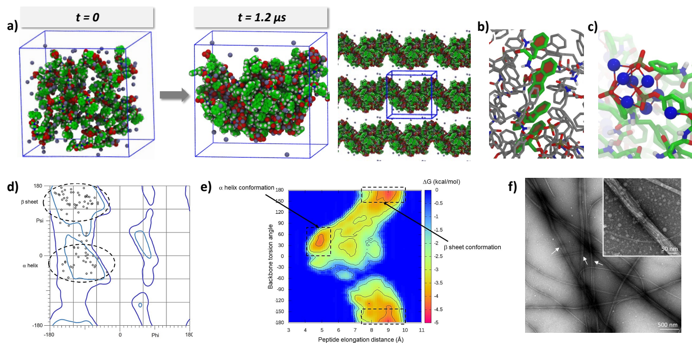
Fig. 4 (a) MD simulations, where 40 Fmoc-FFpY units were randomly arranged in the presence of 500 mM NaCl, at t = 0 (left) and after 1.2 \mu\text{s} dynamics (right), where the 40 peptide units are assembled leading to peptide fibers with this replicated cubic unit. \text{Na}^+ ions are shown in light blue and \text{H}_2\text{O} molecules are hidden for better clarity of the assembly visualization. (b) \pi - \pi stacking of aromatic Fmoc groups in the hydrophobic nucleus of the assembly. (c) Electrostatic interaction between phosphate groups of 3 units Fmoc-FFpY and \text{Na}^+ ions in the outer part. (d) Ramachandran map of one Fmoc-FFpY assembled structure. (e) Conformational free energy landscape of Fmoc-FFpY/ \text{Na}^+ assemblies. (f) TEM micrograph of a negatively stained Fmoc-FFpY6.4/ \text{Na}^+ 500 hydrogel, where arrows marked a helical twisting. The inset shows the zoom-in to visualize the arrangement of fibers forming a nanorod and the helical structure.
