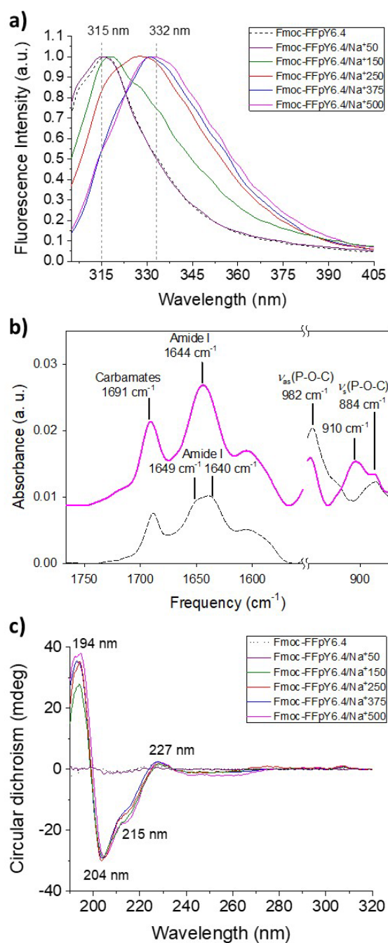
Fig. 2 Fluorescence spectra normalized to the peak at 315 nm, (b) ATR-FTIR spectra, and (c) CD spectra of Fmoc-FFpY in solution in the absence (dashed black curve) and in the presence of different NaCl concentrations: Fmoc-FFpY6.4/Na + 50 (purple curve), Fmoc-FFpY6.4/Na + 150 (green curve), Fmoc-FFpY6.4/Na + 250 (red curve), Fmoc-FFpY6.4/Na + 375 (blue curve), and Fmoc-FFpY6.4/Na + 500 (pink curve).
