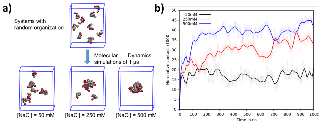
Fig. 3 MD simulations of Fmoc-FFpY in the presence of different NaCl concentrations (a) protocol used and (b) the number of non-native contacts (distance less than 7 Å), along the MD trajectory, between atoms from different peptides. An interpolation using Bézier curves allows us to observe the trend.
