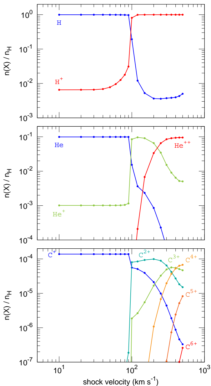
Fig. 9. Fractional abundances of H and \text{H}^+ (top panel), He, \text{He}^+ , and \text{He}^{2+} (middle panel), and \text{C}^+ , \text{C}^{2+} , \text{C}^{3+} , \text{C}^{4+} , \text{C}^{5+} , and \text{C}^{6+} (bottom panel) in the gas entering the shock as functions of the shock velocity. Except for the velocity, all other parameters are set to their standard values (see Table 1).
