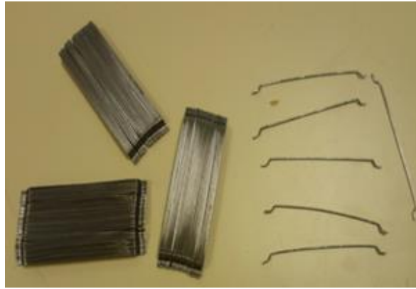
Figure 2. Fibres with end hooks.
