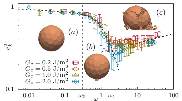
FIG. 9. Squared restitution coefficient e_k^2 as a function of normalized impact energy \omega on a log-log scale for different values of fracture energy G_c . The dotted lines are the fitting forms of Eqs.(13) and (14). The vertical dashed lines mark transition points between different regimes.
