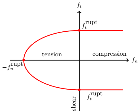
FIG. 4. Strength envelope of a single contact point belonging to an interface between polyhedral primary cells.
