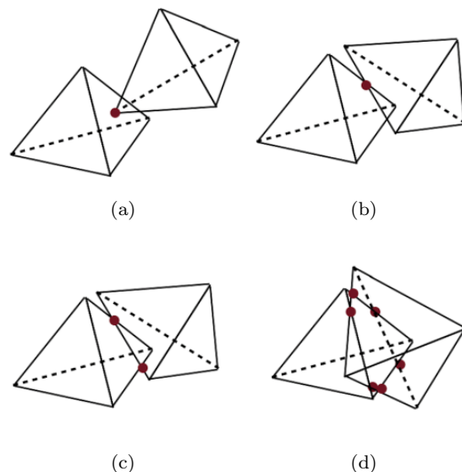
FIG. 3. Different types of contacts between two polyhedra: (a), (b) simple contact, (c) double (edge-face) contact, and (d) triple (face-face) contact.
