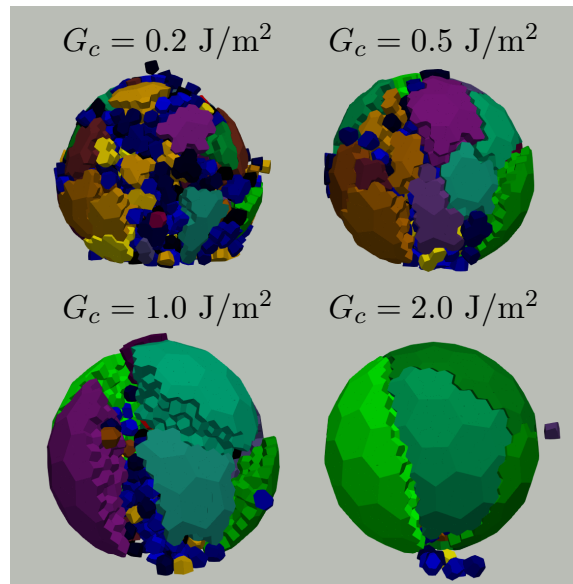
FIG. 6. Fragmentation of a particle impacting a rigid wall for different values of fracture energy G_c . The simulation was carried out with an impact velocity of 4.5 m/s.
