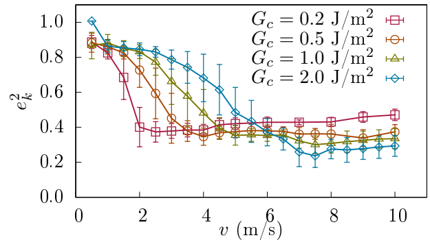
FIG. 8. Squared restitution coefficient e_k^2 as a function of impact velocity v for different values of fracture energy G_c .
