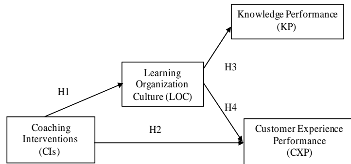
Fig. 6. Research model
