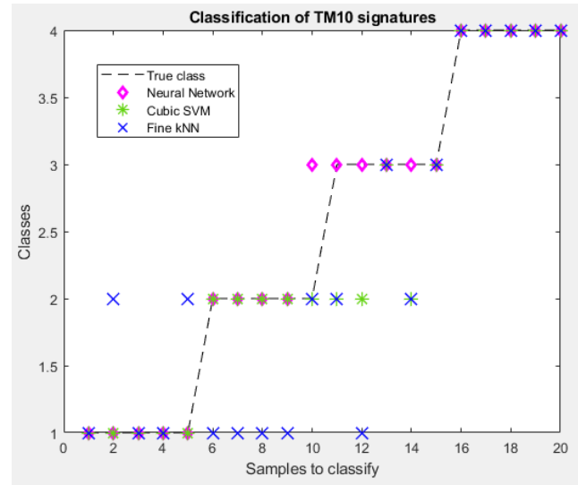
Fig. 7 Classification of 20 signatures from TM10 extracted at known lifetime percentage (0%, 30%, 60% and 100%)
