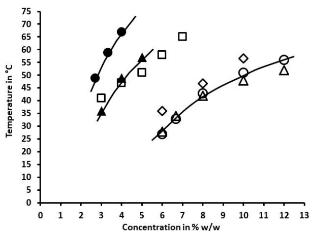
Figure 9. Dependences of the gel → sol transition temperature of gels made from PNAGAs by-products collected from dialysis retentates after enzymatic degradation of different HA-PNAGA in comparison with two PNAGAs of known molar mass (121,000 (◇), and 41,000 (□) g/mol): (△)HA 30 -PNAGA 6, and (○) HA 100 -PNAGA 8 (50% w/w HA in the feed); (▲) HA 30 -PNAGA 1, and (●) HA 100 -PNAGA 2 (20% w/w HA I the feed).
