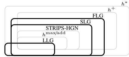
Figure 4: Expressiveness hierarchy of MPNNs on graph representations with respect to STRIPS-HGN and the heuristics h^{\max} , h^{\text{add}} , h^+ and h^* . Bold outlines represent new graphs.
