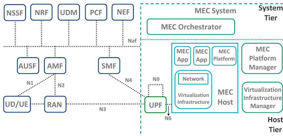
Fig. 4. MEC's integration with 5G network infrastructure.
