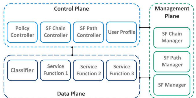
Fig. 8. SFC architecture.
