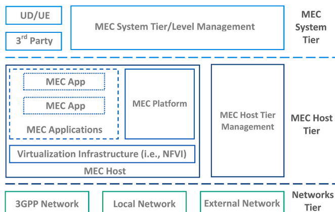
Fig. 2. ETSI MEC framework.
