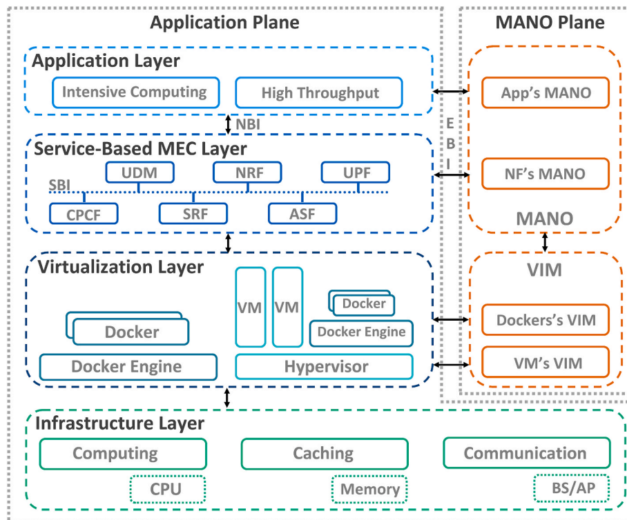
Fig. 16. Open-source MEC framework.
