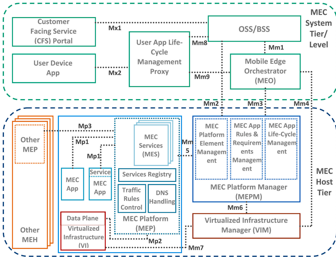
Fig. 3. ETSI MEC reference architecture.
