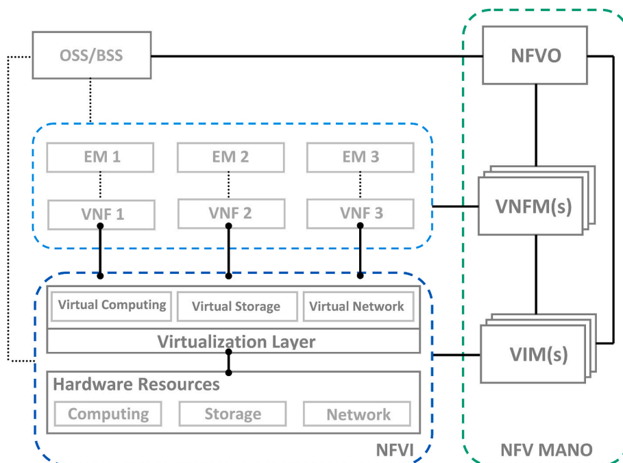
Fig. 5. ETSI NFV architectural framework.
