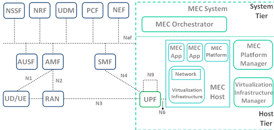
Fig. 4: MEC's integration with 5G network infrastructure.
