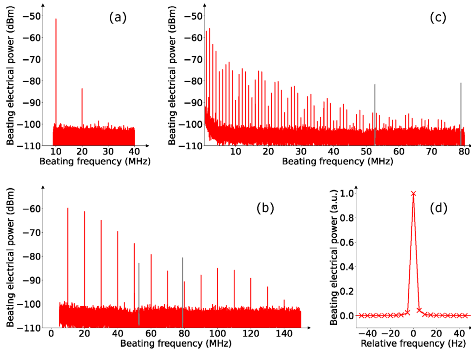
Figure 7. Experimental demonstration of EOFC generation at 8 \mu\text{m} wavelength. a) Beatnote signal coming from the generated EOFC using a CW laser at 8 \mu\text{m} wavelength and a 5 V_{pp} , 10 MHz sinusoidal signal to modulate. b) Beatnote signal measured under the same conditions but using a 20% duty-cycle, 4 V_{pp} square signal. Some parasitic lines, emphasized in grey and coming from the setup could be observed around 53 and 79 MHz. c) Beatnote signal under the same conditions as in b), but using a 1 MHz repetition rate. d) To emphasize the sharpness of the comb lines, a zoom on the first line of the beatnote signal shown in (a) is performed. A FWHM of the beatnote line of 5 Hz is measured, limited by the Doppler resolution, the acquisition time being 0.2 seconds.
