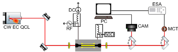
Figure 5. Simplified version of the experimental setup used. The output of a CW external cavity QCL (CW EC QCL) is coupled to the chip using aspheric ZnSe lenses, and collected similarly before being sent to either a mode profiler (CAM) or a fast pre-amplified MCT detector (MCT), whose output is analyzed using an electrical spectrum analyzer (ESA). The modulator is polarised by a SMU (DC) and driven either by an AWG or an ultrafast RF comb generator (RF).
