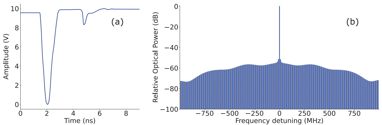
Figure 4. EOFC generation using the RF pulse generator. a) Output pulse of the pulse generator (UltraComb-8G, Ultraview). Its FWHM is 739 ps with a repetition frequency of 10 MHz, with a 10\ V_{pp} amplitude. From simulation, we can expect it to generate the EOFC shown in b) when it is used to drive the modulator.
