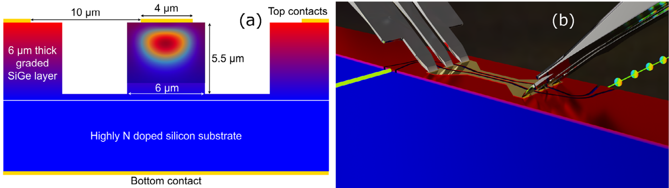
Figure 1. EOFC generation on the graded SiGe platform. a) Cross-section view of the Schottky-based modulator on graded SiGe used. The germanium concentration is represented in colorscale from 0 (blue, pure silicon) to 1 (red, pure germanium) on both sides. The index gradient, similar to the germanium concentration gradient, allows a light confinement close to the Schottky contact as shown in the center, ensuring a large overlap between the optical mode and the voltage dependent space charge region. b) EOFC generation principle. A CW laser source is sent to the modulator, driven by a periodic electrical signal, which modifies both the light amplitude and instantaneous phase and frequency, leading to chirped optical pulses at the output.
