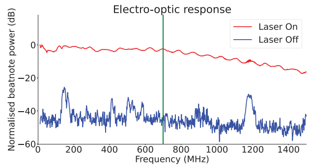
Figure 6. Normalized electro-optic response of the modulator used for the EOFC experiments. The beatnote power is shown in red when the laser is on and in blue when it is off. To emphasize the origin of the drop in the beatnote power, the cut-off of the pre-amplifier of the MCT photodetector is plotted in green.
