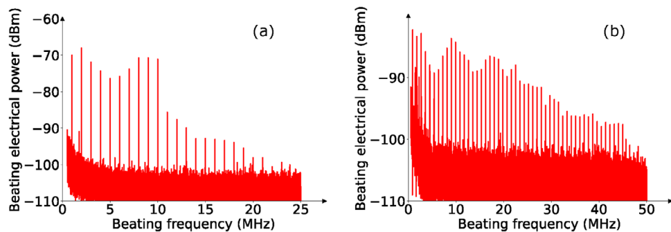
Figure 8. Using sinc -shaped signals to generate EOFC. Resulting beatnote of the generated EOFC using the signal whose expression is given in Equation 2 for a 1 MHz repetition rate and an amplitude of 5 V_{pp} , with a) n = 21 and b) n = 101 .
