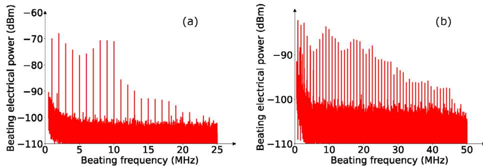
Figure 8. Using sinc -shaped signals to generated EOFC. Resulting beatnote of the generated EOFC using the signal whose expression is given in Equation 2 for a 1 MHz repetition rate and an amplitude of 5 V_{\text{pp}} , with a) n = 21 and b) n = 101 .
