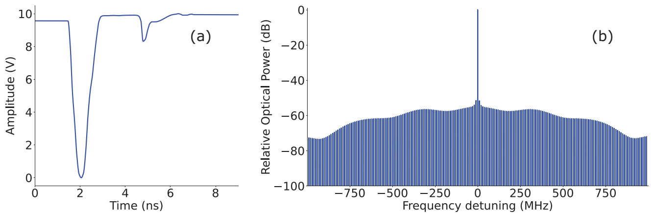
Figure 4. EOFC generation using the RF pulse generator. a) Output pulse of the pulse generator (UltraComb-8G, Ultraview). Its FWHM is 739\ \text{ps} with a repetition frequency of 10\ \text{MHz} , with a 10\ \text{V}_{pp} amplitude. From simulation, we can expect it to generate the EOFC shown in b) when it is used to drive the modulator.
