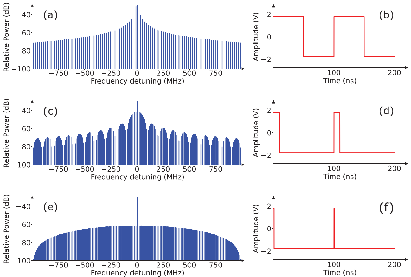
Figure 3. Influence of the varying duty-cycle of a square signal on the output spectrum. a,c,e) Simulated output EOFC around 8\ \mu\text{m} wavelength using 18\ \text{dBm} square signals (corresponding to 0.43\ \text{dB} of extinction ratio) at 10\ \text{MHz} respectively with b) 50\% duty-cycle, d) 10\% duty-cycle and f) 1\% duty-cycle. The central CW line has been cropped for compactness purposes and is always at 0\ \text{dB} .
