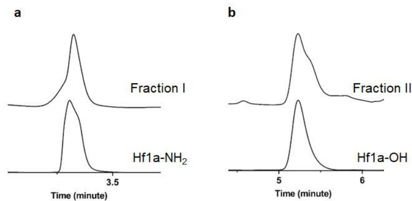
Figure 2. Co-elution of the native and synthetic peptides. (a) Co-elution of native fraction I with synthetic Hf1a-NH 2 . (b) Co-elution of native fraction II with synthetic Hf1a-OH.
