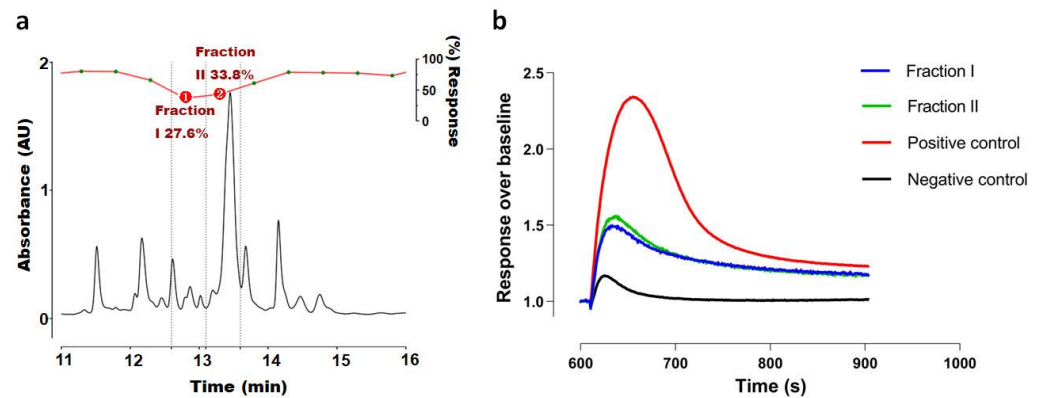
Figure 1. (a) RP-HPLC trace of H. franzweneri fractions (indicated in green points) I and II and their maximum responses at Cav3.2 in the FLIPR assay; (b) Response over baseline traces of the two fractions I and II isolated from scorpion H. franzweneri , showing 72.4% and 66.2% inhibition of \text{Ca}^{2+} responses in Cav3.2, respectively.
