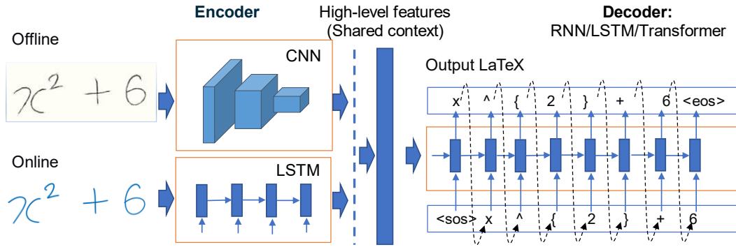
Fig. 5. General architecture of an encoder–decoder model. Dashed arrows show output of previous steps being used as input for the next step. <eos> - end of string, <sos> - start of string.
