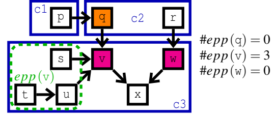
Figure 3: Illustration of the \#ep(b) metric.
