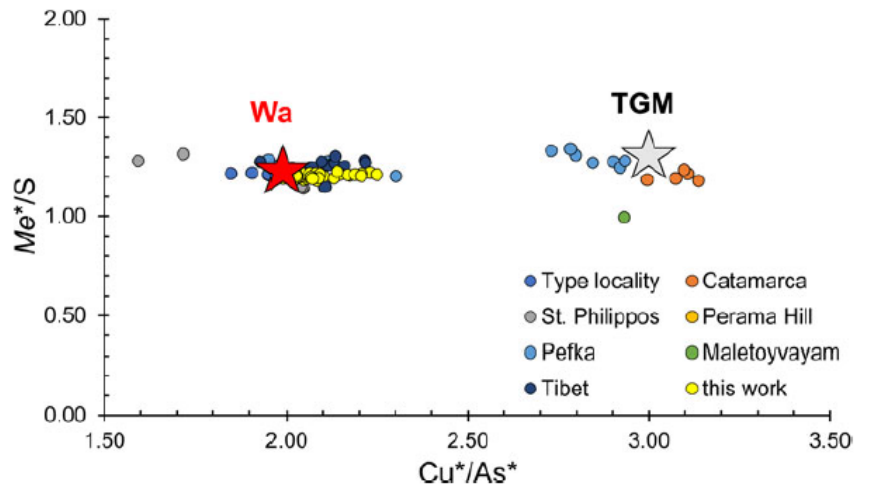
Figure 2. Diagram showing the relation between \text{Cu}^*/\text{As}^* vs. \text{Me}^*/\text{S} ratios for samples of watanabeite described in literature. Red and grey stars indicate the ideal values for watanabeite (Wa) and tetrahedrite-group minerals (TGM). Chemical data are after Shimizu et al. (1993) for the type locality; Paar et al. (2002), Makovicky et al. (2005), and Márquez-Zavalía and Galliski (2007) for Catamarca province, Argentina; Voudouris et al. (2005) for St. Philippos, Greece; Voudouris et al. (2011) for Perama Hill, Greece; Repstock et al. (2015) for Pefka, Greece; Sidorov et al. (2020) for Maletoyvayam, Russia; Zheng et al. (2021) for the Jiama porphyry system, South Tibet. Yellow circles represent analytical data from our study.
