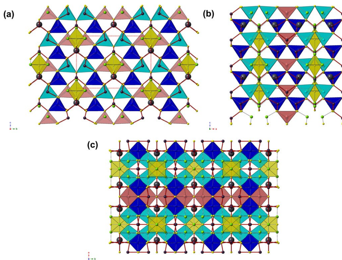
Figure 4. Crystal structure of watanabeite as seen down [100] (a), [010] (b), and [001] (c). Polyhedra: dark blue = Cu(1) site; light blue = Cu(2) site; pink = Cu(3) site; yellow = S(8) site. Circles: green = Cu(4)-Cu(6) sites; violet = As(1)-As(3) and M(1a) sites; dark grey = M(1b) site; yellow = S(1)-S(7) sites. Red dotted lines indicated the unit cell, drawings made using CrystalMaker® software.
