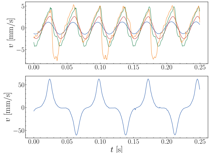
Figure 5: Top: Temporal evolution of the horizontal velocity of the magnet, for increasing plate amplitudes A (in order blue, red, green, yellow) at fixed f = 27 Hz, and below the period-doubling instability threshold (white area in Fig. 3). Bottom: same within the period-doubling region (red area in Fig. 3).
