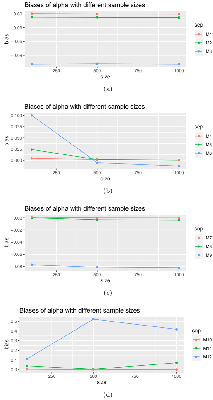
Figure 18: Comparing biases of parameter estimations for \alpha (rate for the exponential component)
