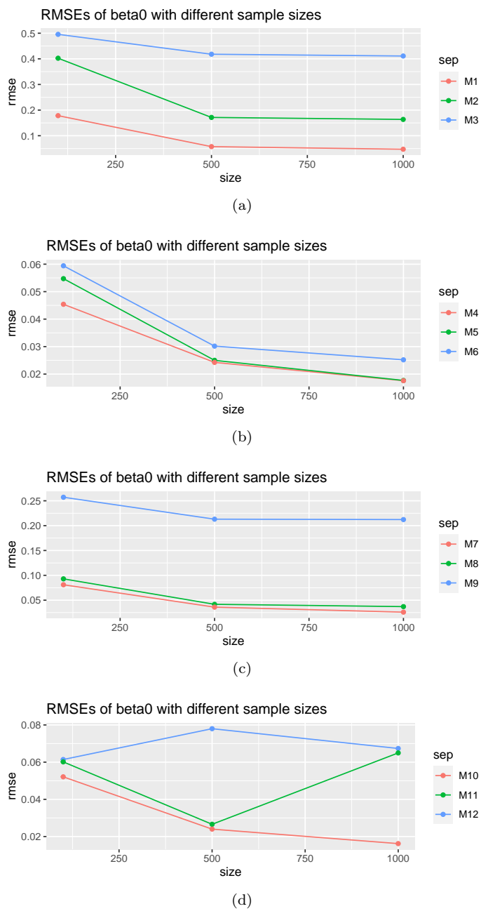
Figure 9: Comparing RMSEs of parameter estimations for \beta_0 (the intercept)
