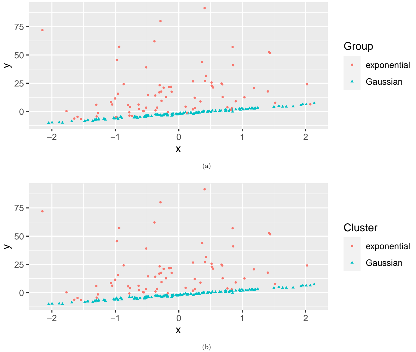
Figure 2: (a) Scatter plot of the simulated data assuming a flare regression model with two components labelled ( n=200 , x \sim N(0, 1) , \lambda = 0.6 , \beta = (-2, 4) , \sigma = 0.5 , and \alpha = 0.05 ) and (b) scatter plot of the same simulated data with clusters labelled (cut-off probability equals to 0.8)
