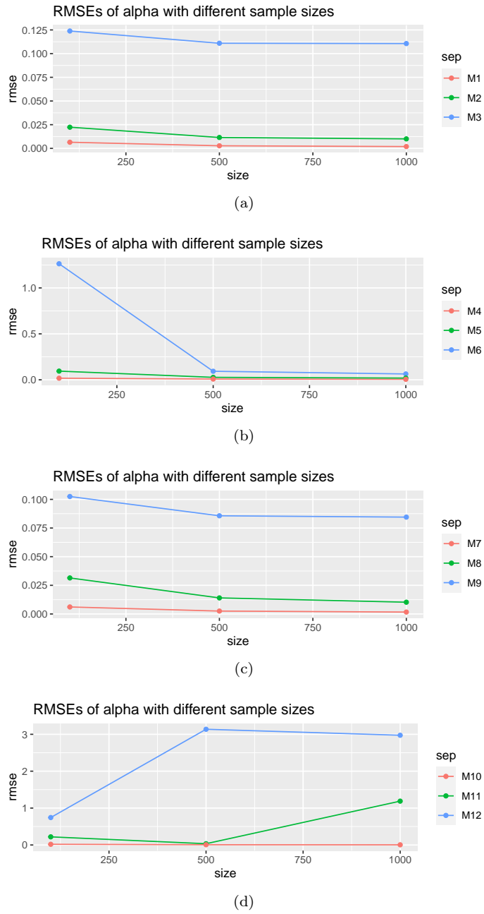
Figure 17: Comparing RMSEs of parameter estimations for \alpha (rate for the exponential component)
