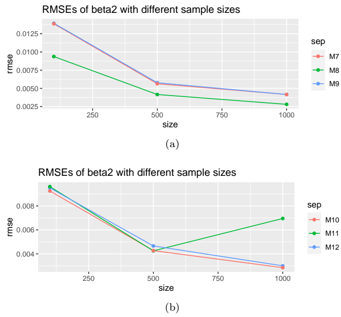
Figure 13: Comparing RMSEs of parameter estimations for \beta_2 (regression coefficient 2)
