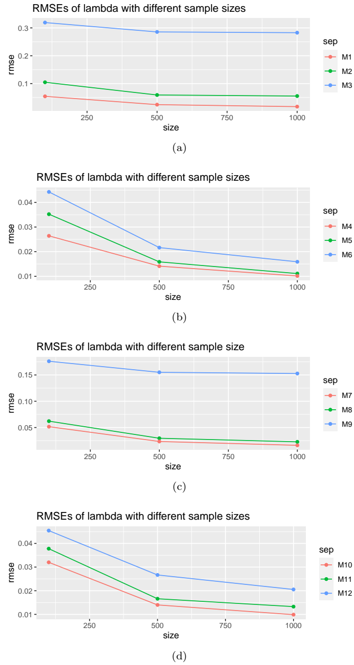
Figure 7: Comparing RMSEs of parameter estimations for \lambda (the mixing proportion)
