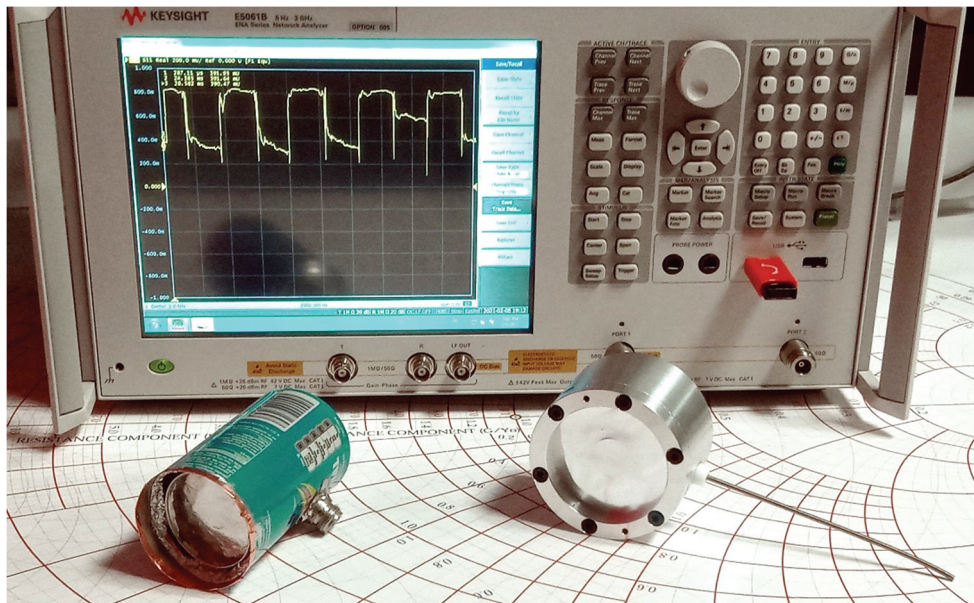
Fig.6. Measurement of S11 in Zero Span mode using the network analyzer of the device built by students from a soda can and kitchen aluminum foil: During the measurement, the membrane is alternately pressed or disconnected from the metal rod constituting the coaxial cavity.
