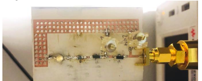
Fig. 3. The Harmonic Doubler Reflection Amplifier.
