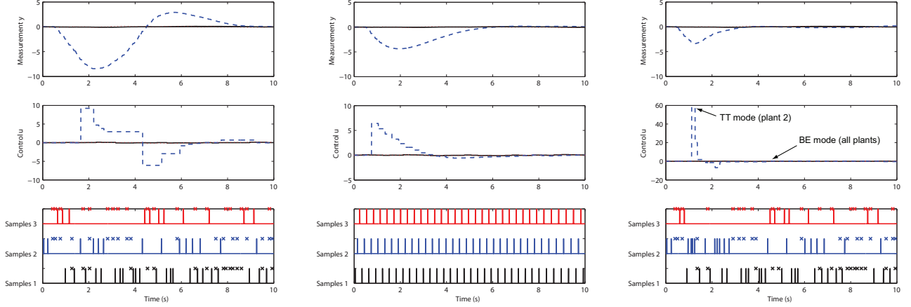
(a) Pure CA MAC scheme with control law L_0 in (b) Pure CF MAC scheme with control law L_0 in (c) Hybrid MAC scheme with hybrid control law BE mode, and \alpha = 0.33 . TT mode and sampling period 0.3.
