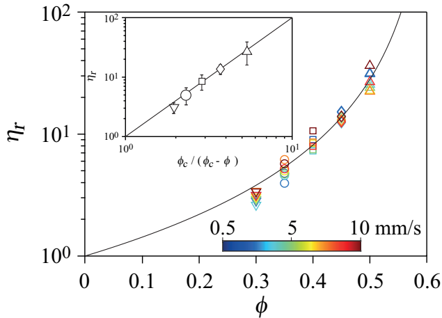
Figure 3. Relative viscosity of the suspension versus the particle volume fraction \phi in semi-log scale. The imposed velocity V_0 ranges from 0.5 up to 10 \text{mm}\cdot\text{s}^{-1} and the magnitude of the velocity is in agreement with the colorbar. The solid line corresponds \eta_r = (\phi_c / (\phi_c - \phi))^2 with \phi_c = 0.61 . Inset: Relative viscosity of the suspension versus reduced volume fraction (\phi_c / (\phi_c - \phi)) . Each symbol is the average of the relative viscosity for the different velocities.
