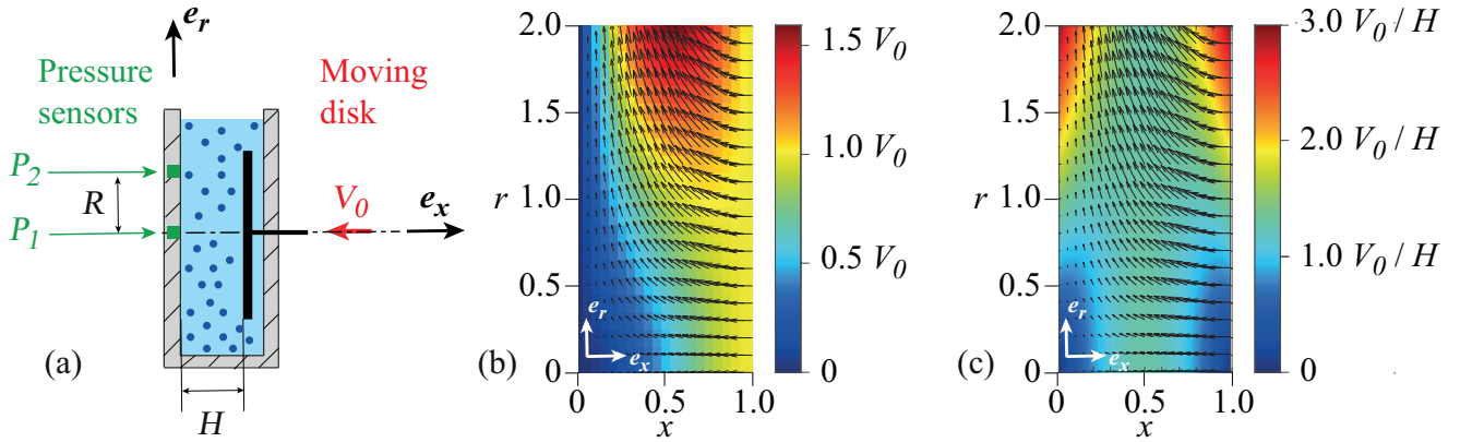
Figure 1. a Sketch of the experimental setup: a moving disk is squeezing the suspension at a constant velocity V_0 along e_x . Pressure sensors are located on the opposite wall in order to measure the pressure difference P_1 - P_2 . b Velocity field associated to the squeeze flow deduced from Eqs. (7) and (8). The color map represents the norm of the velocity. c Shear rate field associated to the squeeze flow according to Eqs. (7) and (8). The color map represents the shear rate calculated from Eq. (13). The black arrows represent the velocity field as in figure b.
