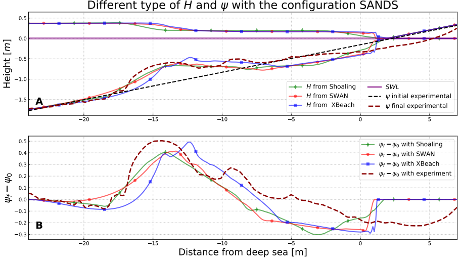
Figure 7: A) Hydro-Morphodynamic results obtained with OptiMorph model using Hadamard strategy with wave models (Shoaling (green), SWAN (red) and XBeach (blue)). Bottom profile configuration from the SANDS erosive experience. Black: bottom profile, green: H and \psi from improved shoaling with Hadamard strategy, red: H and \psi from SWAN with Hadamard strategy, blue: H and \psi from XBeach with Hadamard strategy, dark red: \psi from experience. B) Morphodynamic ecarts of \psi_f - \psi_i obtained with the Shoaling, SWAN, XBeach models and experiment. Bottom profile configuration from the SANDS channel experiment. In green: morphodynamic differences from shoaling with Hadamard strategy ( \psi_{RMSE} = 11.7 cm), red: morphodynamic differences from SWAN with Hadamard strategy ( \psi_{RMSE} = 12.7 cm), blue: morphodynamic differences from XBeach with Hadamard strategy ( \psi_{RMSE} = 13.5 cm), dark red: morphodynamic differences from the experiment.
