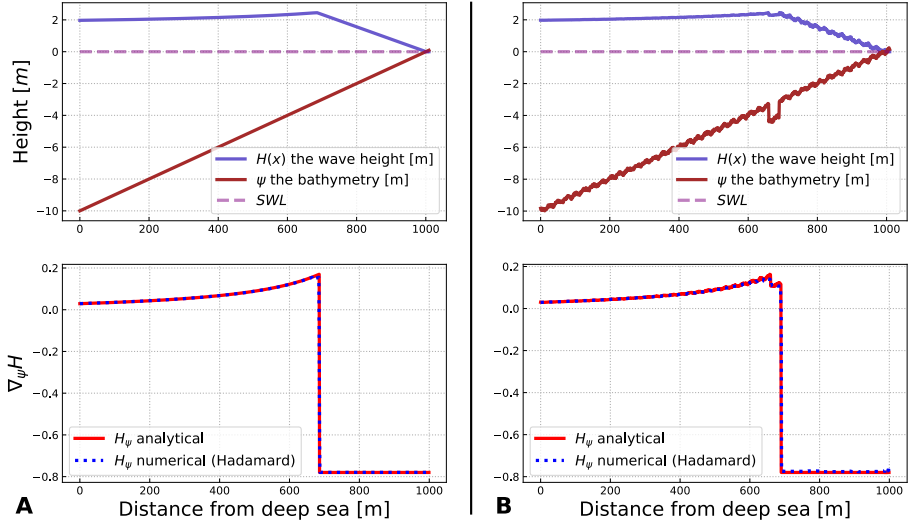
Figure 5: Comparison of numerical and analytical solution of \nabla_{\psi}H using OptiMorph model. Configuration without (A) / with (B) perturbations, H_0 = 2 m, h_0 = 10 m and the wave period T_0 = 10 s. In dodgerblue, the wave height H , in brown the bottom profile \psi , in red \nabla_{\psi}H calculated analytically, in blue \nabla_{\psi}H calculated by Hadamard strategy.
