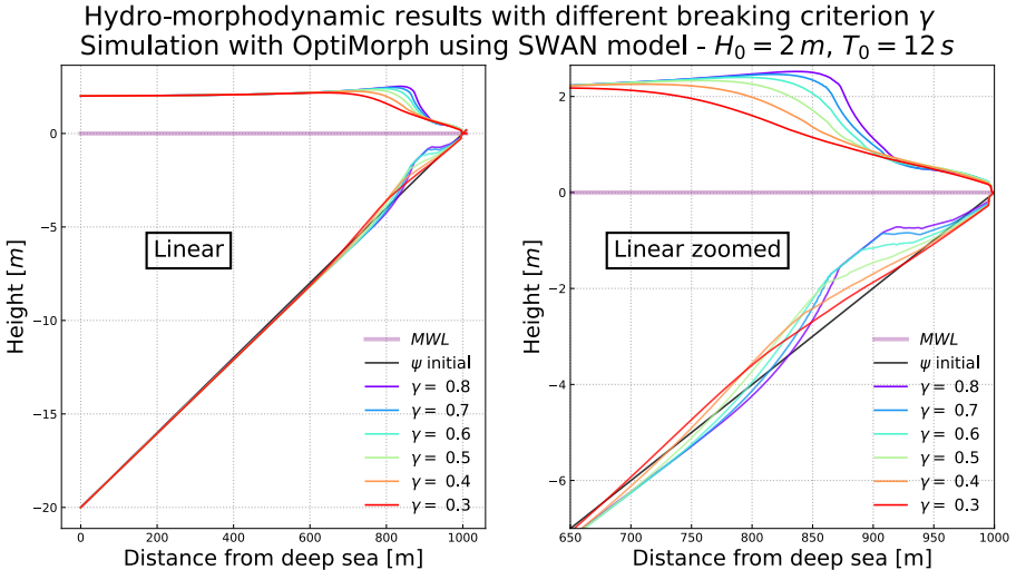
Figure 11: Hydro-morphodynamic results with different breaking criterion \gamma - Simulation with OptiMorph (Hadamard strategy) using SWAN model - H_0 = 2 m, T_0 = 12 s, h_0 = 20 m.
