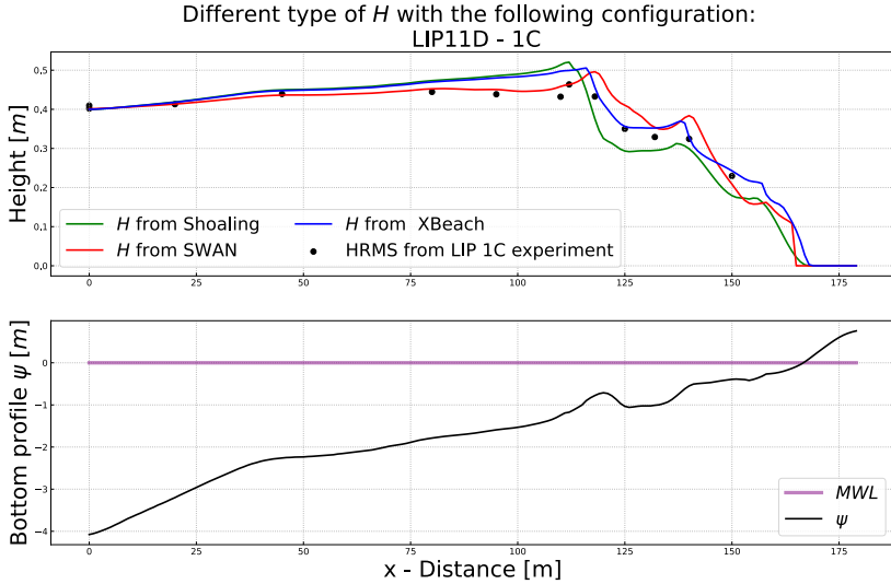
Figure D3: Wave results obtained with the Shoaling, SWAN and XBeach models. Sea bottom configuration from the LIP 1C channel experiment. Black points, measured HRMS, black bottom profile, green H from extended shoaling ( H_{RMSE} = 0.045 m), red H from SWAN ( H_{RMSE} = 0.033 m), blue H from XBeach ( H_{RMSE} = 0.028 m).
