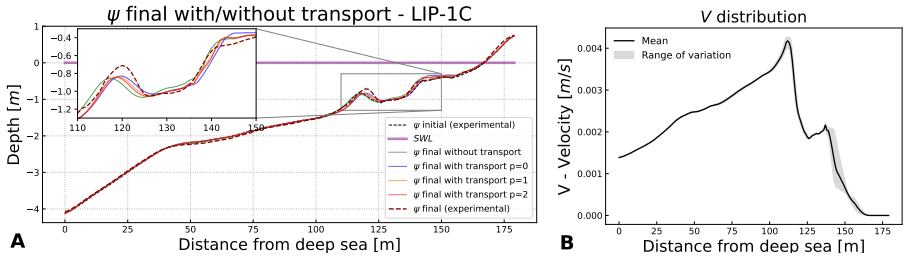
Figure 10: A) Morphodynamic results by the OptiMorph model augmented by the transport mechanisms for p = 0, 1, 2 and the XBeach wave model, for the LIP 1C channel experiment. B) Velocity distribution for p = 1 .
