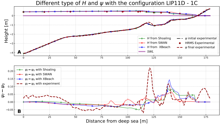
Figure 8: A) Hydro-Morphodynamic results obtained with OptiMorph model using Hadamard strategy with wave models (Shoaling (green), SWAN (red) and XBeach (blue)). Bottom profile configuration from the LIP 1C channel experiment. Red points: measured HRMS, black: bottom profile, green: H and \psi from improved shoaling with Hadamard strategy, red: H and \psi from SWAN with Hadamard strategy, blue: H and \psi from XBeach with Hadamard strategy, dark red: \psi from experience. B) Morphodynamic ecart of \psi_f - \psi_i obtained with the Shoaling, SWAN, XBeach models and experiment. Bottom profile configuration from the LIP 1C channel experiment. In green: morphodynamic differences from shoaling with Hadamard strategy, red: morphodynamic differences from SWAN with Hadamard strategy, blue: morphodynamic differences from XBeach with Hadamard strategy, dark red: morphodynamic differences from the experiment.
