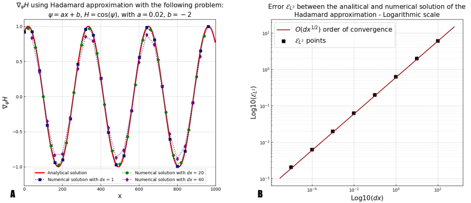
Figure 4: A) Calculation of \nabla_{\psi} H using Hadamard approximation with the following problem (see C.2): \psi = ax + b , H = \cos(\psi) , with a = 0.02 , b = -2 . B) L^2 error and order of convergence for a comparison between the analytical solution of the simple problem described in C.2 with H = \cos(\psi) .
