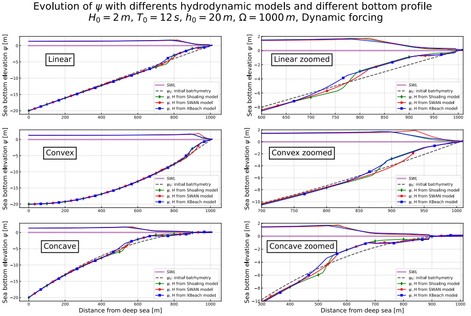
Figure 9: Evolution of \psi using Hadamard strategy with extended Shoaling (green), SWAN (red) and XBeach (blue) models. Simulation on open-sea configuration with linear, convex and concave configurations. Simulation parameters of H_0 = 2 m, T_0 = 12 s, h_0 = 20 m, \Omega = 1000 m.
