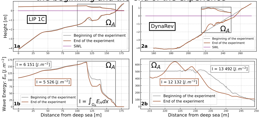
Figure 2: 1) LIP 1C experiment with H generated by XBeach. 2) DynaRev experiment with H measured by LIDAR. a) Bottom profile and averaged water height at the beginning of the experiment (grey), Bottom profile and averaged water height at the end of the experiment (brown). b) Wave energies associated with water heights. The energy is calculated on the black rectangle \Omega_A .
