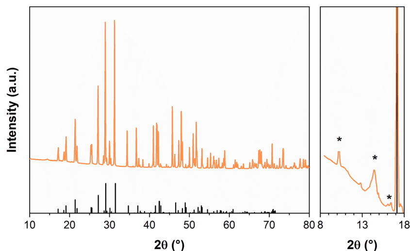
Fig. 8 SPXRD pattern obtained for \text{Nd}_{0.8}\text{Ca}_{0.1}\text{U}_{0.1}\text{PO}_4 monazite–cheralite converted in air at 1100^\circ\text{C} for 6 hours. PXRD patterns reported for monazite \text{NdPO}_4 (black vertical bars); 40 * indicates additional peaks observed in the experimental pattern.
