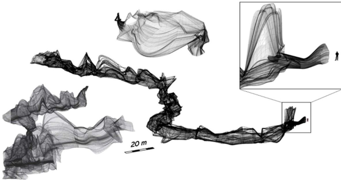
Figure 9. 3D models of the three show caves resulted from the proposed techniques. The caves include Muang-On (lowermost), Chiang-Dao (middle), and San-Han (uppermost). An additional scale is presented as a human with a height of 1.7 m showing in the extended square area. The user-interactive version of the Muang-On and Chiang-Dao cave 3D models are published via Sketchfab.
