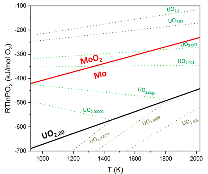
Fig. 8. Ellingham diagram showing the Mo/MoO 2 (data from [26]) equilibrium oxygen potentials with several \text{UO}_{2\pm x} examples (data from [43]), including exact \text{UO}_{2.00} .
