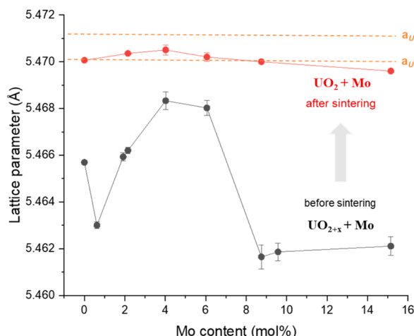
Fig. 3. Calculated lattice parameter values (Å) of the uranium oxide structure obtained after hydroxide conversion (in black) and after sintering (in red) as a function of Mo content (mol%). Examples of lattice parameter measurements of stoichiometric \text{UO}_{2.00} are represented in dashed lines: a = 5.47127 \pm 0.00008 Å by G. Leinders et al. [32] and a = 5.4704 \pm 0.00008 Å by F. Grønvold [33].
