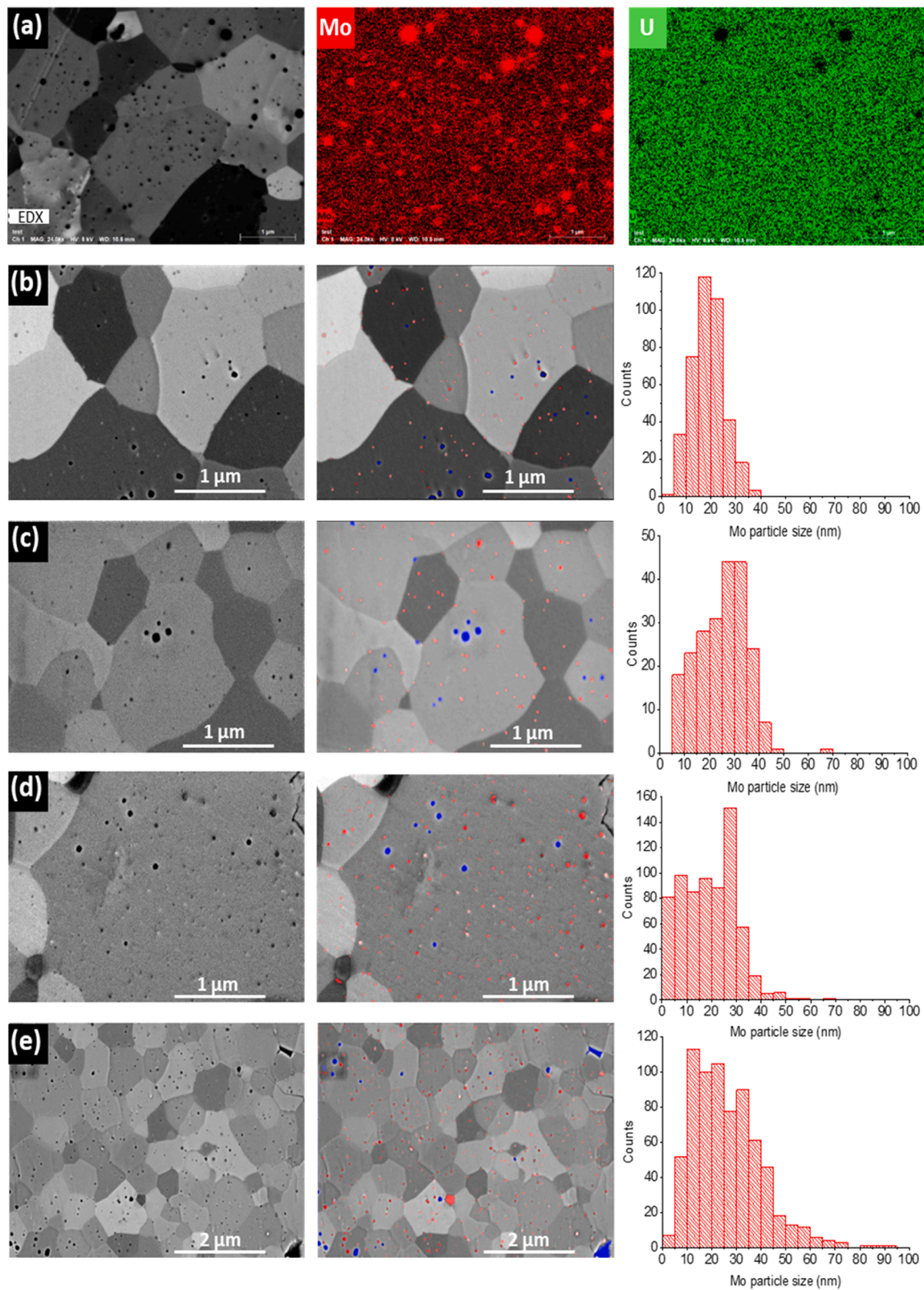
Fig. 5. (a) EDS mapping images of a polished \text{UO}_2 + 9 \text{ mol\% Mo} sample pellet; (b), (c), (d), and (e): high magnification SEM-BSE image examples recorded at 3 kV of selected zones in the polished samples for determining Mo particle size distribution by Trainable Weka Segmentation at Mo contents 2, 4, 6, and 9 mol% in \text{UO}_2 , respectively. The Mo particles are red-colored, and the pores are blue-colored.
