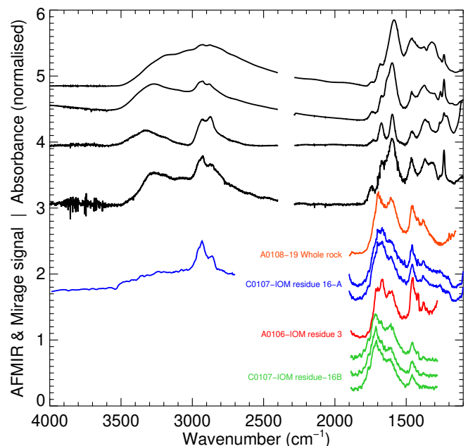
Fig. 10. Comparison of AFM-IR and O-PTIR (mIRage ® ) spectra of nanoglobule-like inclusions from this study with IR spectra of some macromolecular residues from Muñoz Caro & Schutte (2003) , obtained after irradiation of interstellar ice analogues and annealing to room temperature. These irradiation experiments simulate the physical conditions in dense clouds and the accretion and photoprocessing of ices on grain surfaces.
