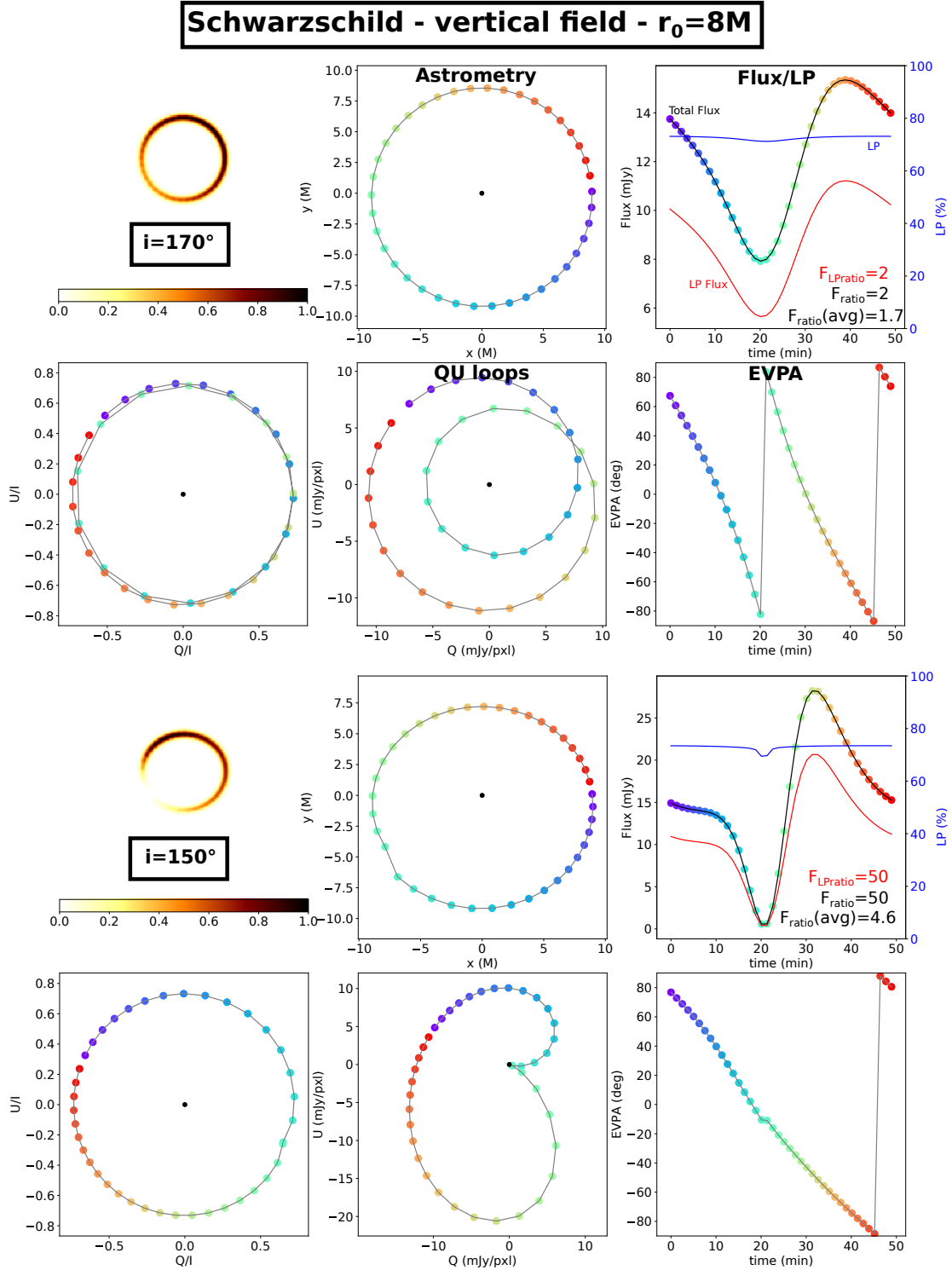
Fig. 10. Same as Fig. 7 but in Schwarzschild spacetime for a vertical magnetic field. It might seem surprising that there is a small kick on the astrometric path toward the southeast. This is due to the dependence of the radiative transfer coefficients on \sin \theta_B , where \theta_B is the angle between the direction of the magnetic field and the direction of emission (see Marszewski et al. 2021). The upper-left panel clearly shows a flux depletion toward the southeast due to this effect. At this orbital phase, the direction of emission in the emitter’s frame, \mathbf{K} , becomes vertical and parallel to the magnetic field. Due to the combination of special-relativistic aberration and general-relativistic lensing effects, the direction of \mathbf{K} varies with the orbital phase. The QU loops of this figure should be compared to that of Fig. 7, as the similarity is striking.
