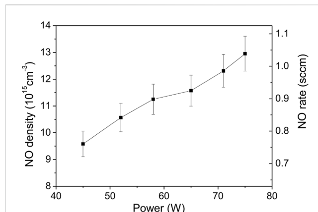
FIGURE 13 NO density function of power for air/Ar molar ratio of 10% and total flowrate of 2 NL/min.
