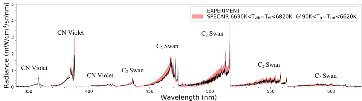
Figure 7 Comparison between experimental spectrum and SPECAIR prediction at the exit of the torch over the CN Violet and C_2 Swan vibrational bands with 6690 < T_{vib} = T_{el} < 6820 K and a slightly reduced temperature translational/rotational temperature of 6490 < T_{tr} = T_{rot} < 6620 K.
