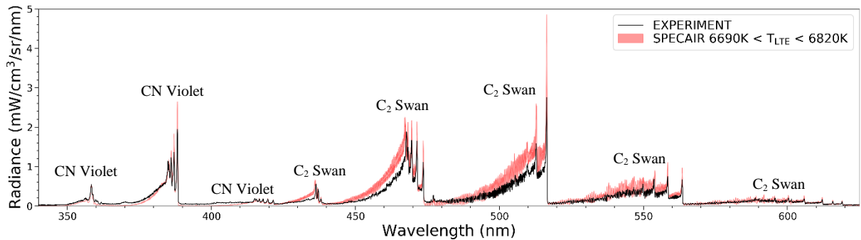
Figure 5 Comparison between experimental spectrum and SPECAIR prediction at the exit of the torch over the CN Violet and C_2 Swan vibrational bands 6690 < T_{LTE} < 6820 K.
