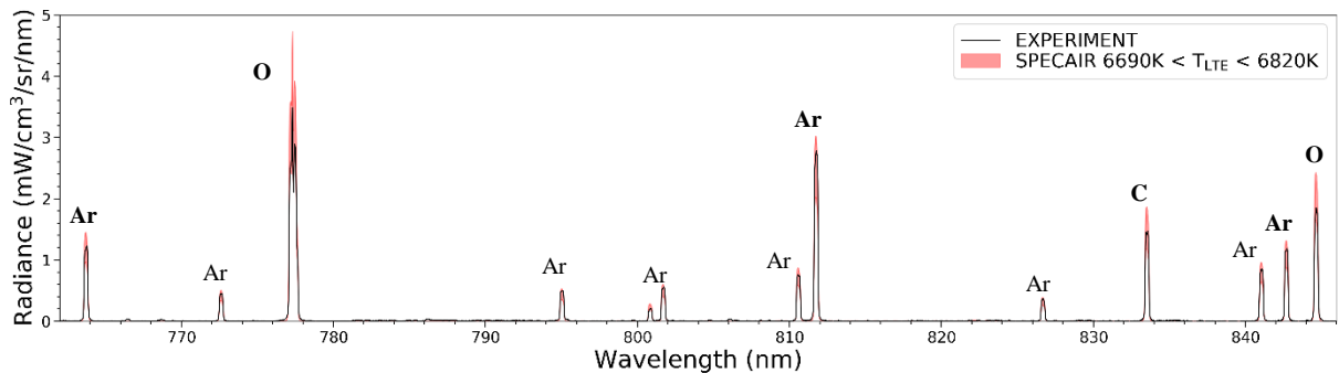
Figure 6 Comparison between experimental spectrum and SPECAIR prediction at the exit of the torch of the atomic lines of argon, carbon and oxygen 6690 < T_{LTE} < 6820 K.
