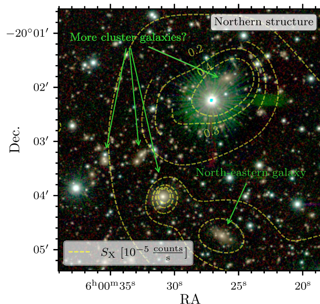
Figure 9. A 4.8 \text{ arcmin} \times 4.8 \text{ arcmin} cut-out of the VIRCAM colour-composite image used in Fig. 2 (blue: Y band, green: J band, red: Ks band) showing the northern X-ray emission structure (see left-hand panel of Fig. 6). The X-ray surface-brightness contours are overlaid in yellow as in Fig. 1. The X-ray emission in this region concurs with an overdensity of galaxies that match the colours of cluster members, suggesting that it likely lies at the same redshift as the cluster.
