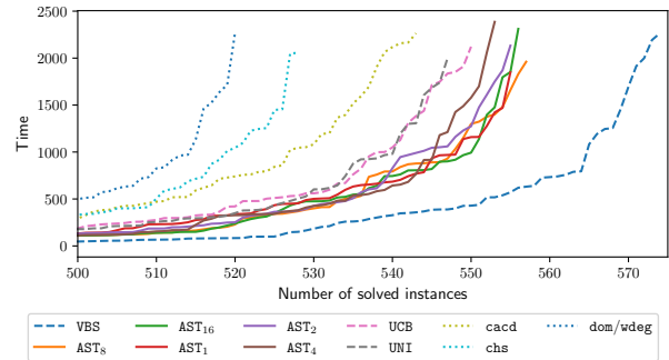
Figure 2: Cactus plots of the best branching strategies.
