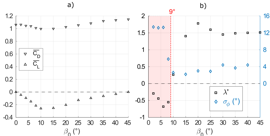
Figure 4: a) Evolution of the mean static drag and lift coefficients \overline{C_D} and \overline{C_L} with the static yaw angle of the cube \beta_0 for U_0 = 15 \text{ m/s} for the S120 setup b) Reduced aerodynamic damping coefficient \lambda' of the tethered cube and standard deviation \sigma_\phi of the angle \phi derived from measurements at U_0 = 15 \text{ m/s} for different static yaw angles \beta_0 for the S120 setup ; the red area shows the unstable region
