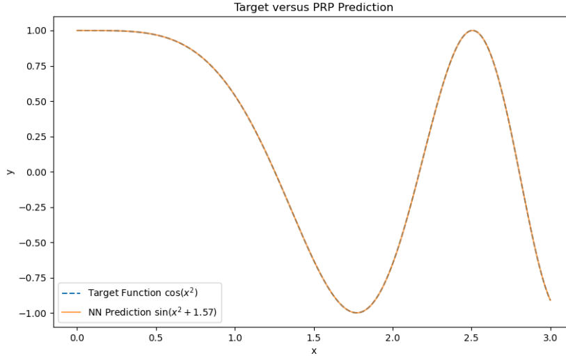
FIGURE 4. Case 2: comparison of the results from the PRP-Nested SINDy, which yielded the function x \mapsto \sin(x^2 + 1.57) , with the target function x \mapsto \cos(x^2) , over the interval [0, 3] .
