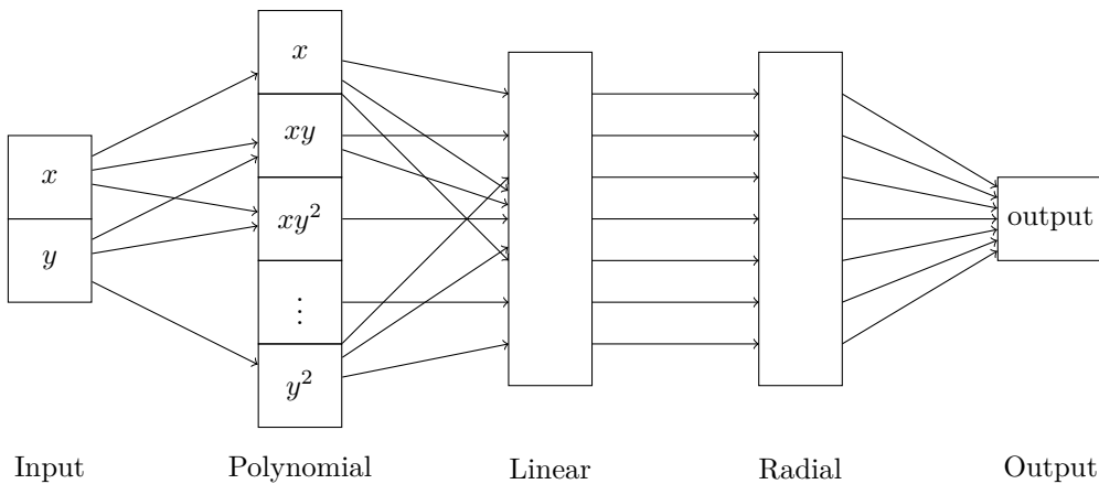
FIGURE 1. Structure of the PR model for d = 2 and 2 input variables.
