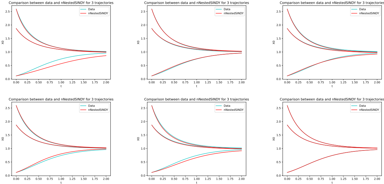
(B) We compare trajectories of dynamic systems (5.5) (red curves) and (5.7) (blue curves) for three different initial conditions, at epochs 50, 150, 300, 1000, 1500, 1900 (from left to right and top to bottom)
