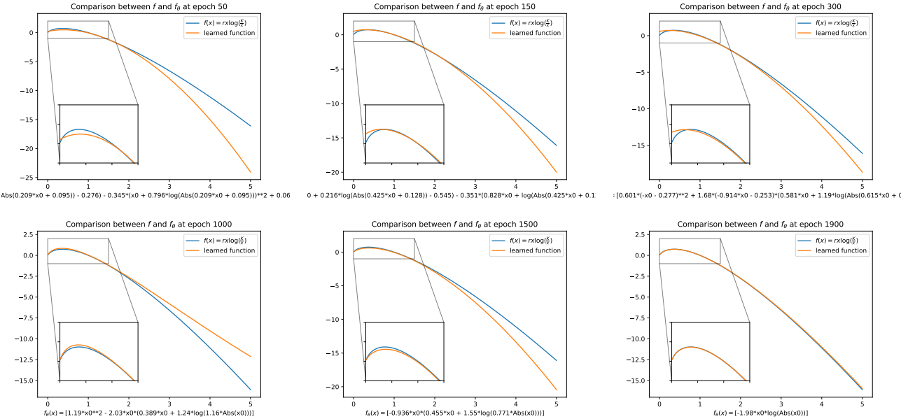
(A) We compare f given by (5.8) (blue curve) and the learned function f_\theta (orange curve), at epochs 50, 150, 300, 1000, 1500, 1900 (from left to right and top to bottom)
