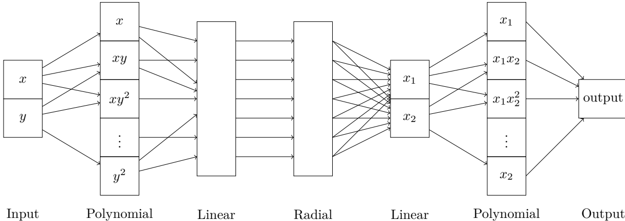
FIGURE 2. Structure of the PRP model for l = 2 , d = 2 , and 2 input dimensions.
