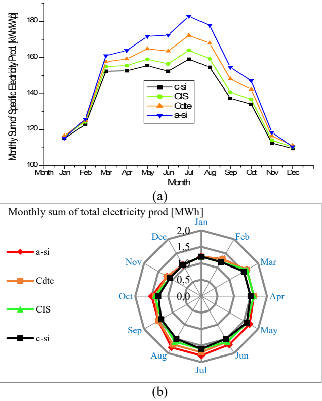
Figure 8. (a) Monthly sum of specific energy, (b) total electricity production for each PV technology
